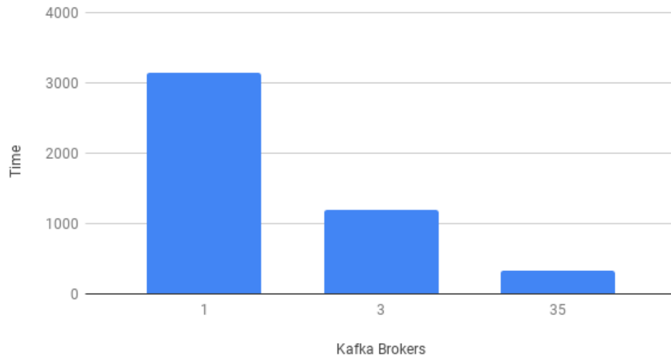
Figure 2: Completion time of sensor data ingestion
