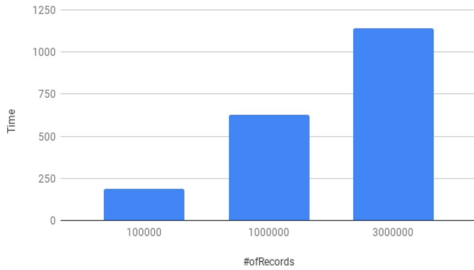
Figure 18: Completion time of enriched data ingestion
