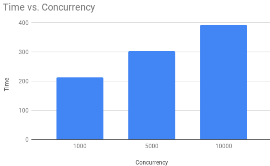
Figure 14: Completion time of dataset upload step
