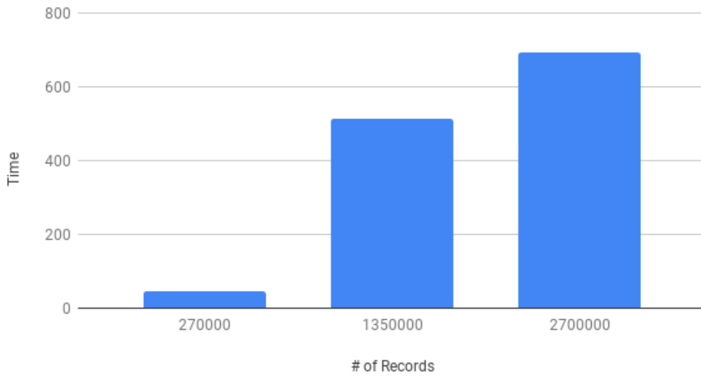
Figure 46: Completion time for the ingestion of semantically enriched data
