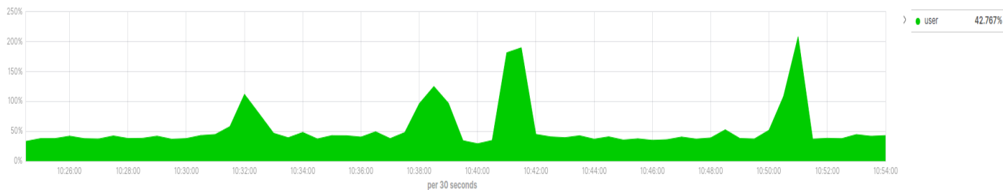
Figure 39: CPU usage during ingestion of enriched data
