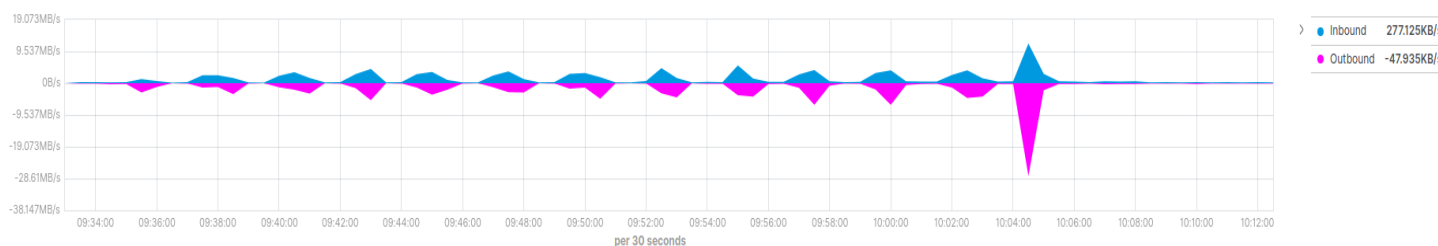
Figure 36: Network usage during data streams pipeline
