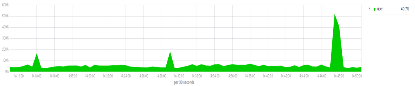
Figure 19: CPU usage during ingestion of enriched data
