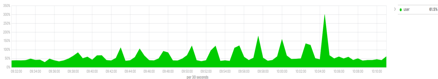
Figure 35: CPU usage during data streams pipeline
