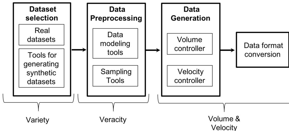
Figure 3: The big data generation process
