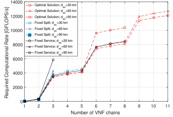
Figure 4. Required computational rate for different VNF deployment schemes with respect to the number of supported VNF chains. C^c=8960 GFLOPS/s and C^e=4480 GFLOPS/s.
