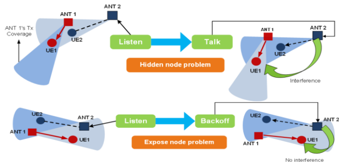
Figure 2 Example of hidden and exposed node problems in HF.
