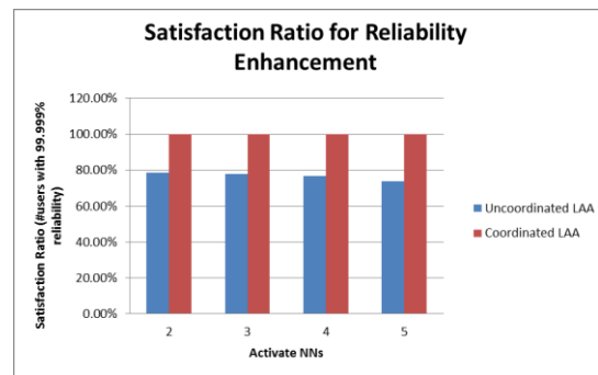
Figure 5 Satisfaction Ratio for Reliability enhancement.
