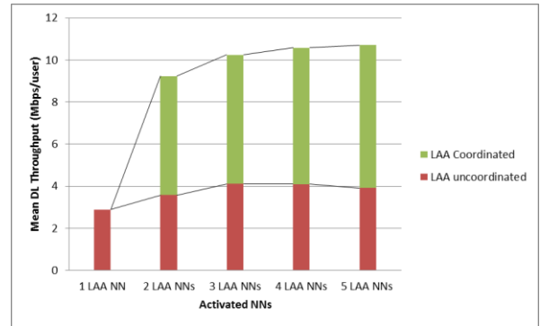
Figure 4 Mean User Throughput for different LAA NN Activations.
