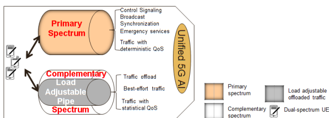
Figure 1 Joint operation of 5G NR on both licensed and unlicensed bands. Air interface is denoted by AI in the figure.
