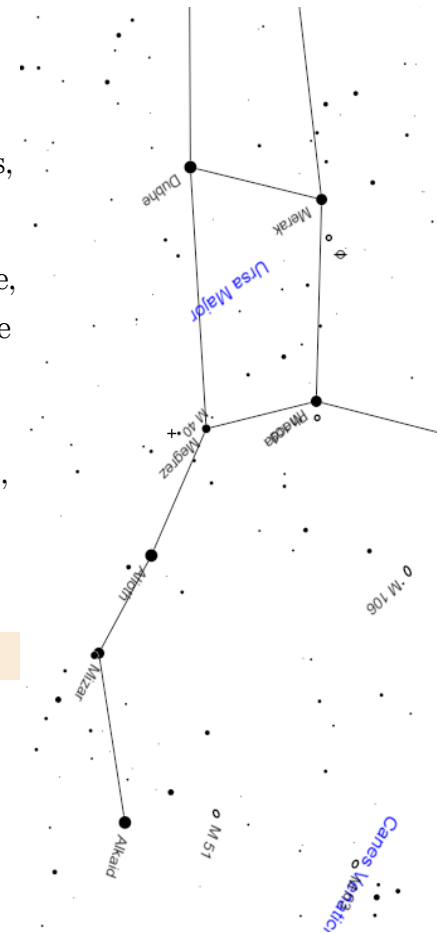
Figure 15: View of Big Dipper in current era
