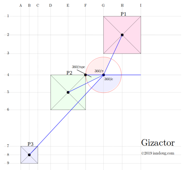
Figure 40: Selected points from the G4 connections between P1, P2 and P3
