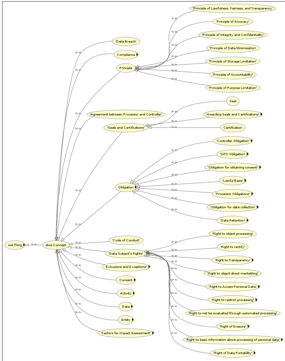
Fig. 3: (a) Terms defined under GDPRtEXT using SKOS
