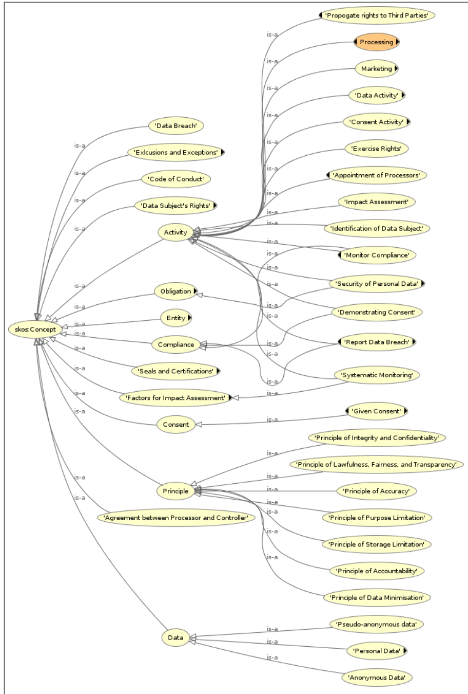
Fig. 3: (b) Terms defined under GDPRtEXT using SKOS
