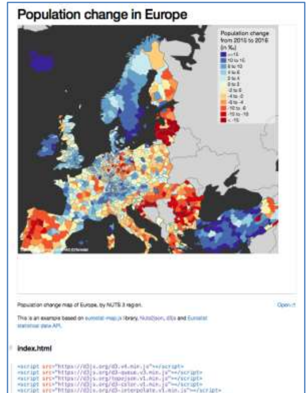
Figure A: Examples of DIY services for Eurostat open data. Left: happyGISCO allows the user to run GISCO web-services and query its API directly from a ready-to-use interactive computing platform (e.g., a Jupyter notebook distributed through a docker virtualised container); in that case, NUTS datasets are fetched and used as-is into the full-stack operation. Right: eurostat-map.js provides with a set of reusable cartographic styles for showing genuine Eurostat figures. These styles concern choropleth maps, proportional symbol maps, categorical maps, etc. ; in this example, a map population change over Europe is generated in a web page and the script to reproduce the map is also provided; note that this library uses the NUTS2json tools which provide reusable web-formatted versions of NUTS datasets.
