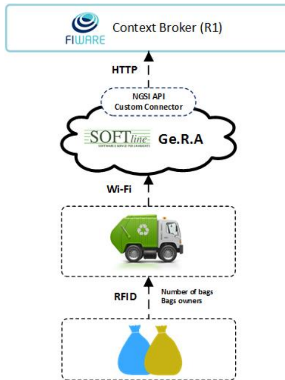
Figure 47. Conceptual communication architecture of the SEVESO sensors.
