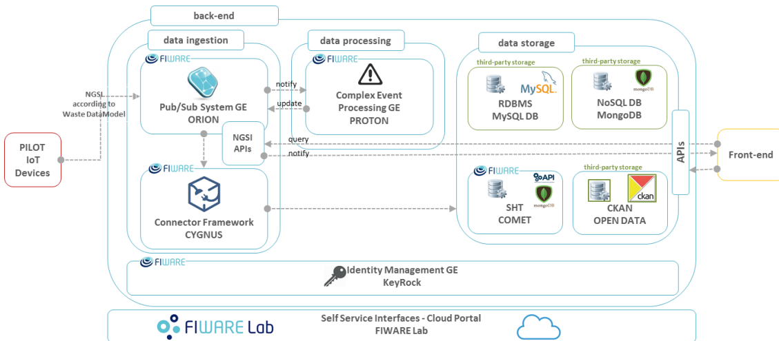
Figure 10. Conceptual back-end architecture.
