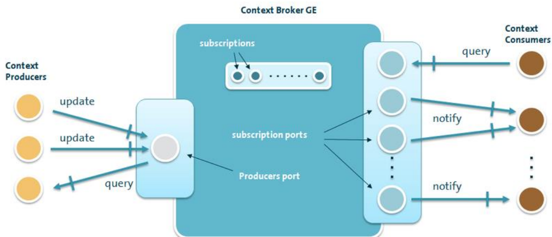
Figure 11. Logical architecture of the Publish/Subscribe Context Broker GE.
