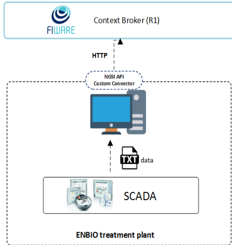
Figure 48. Conceptual communication architecture of the ENBIO treatment plant.
