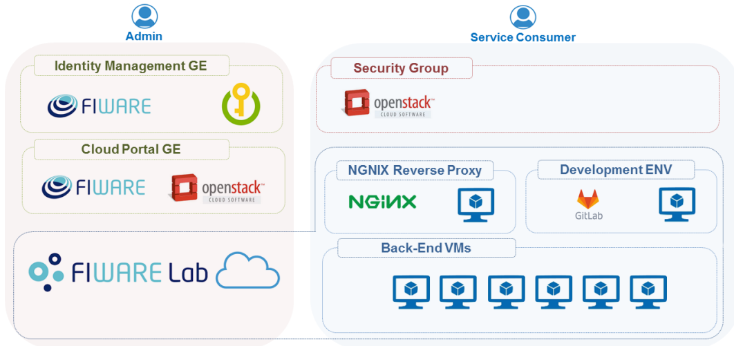
Figure 4. Physical architecture.
