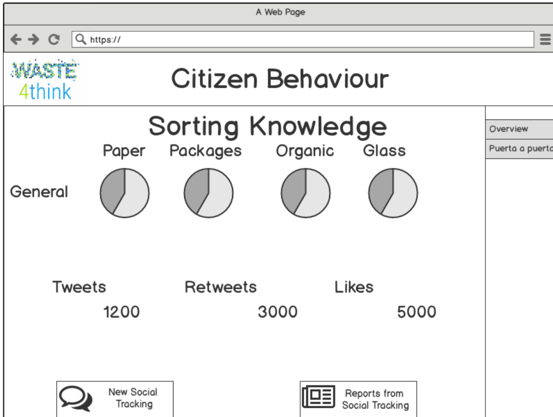
Figure 42. Main view of the Citizen Behaviour Tracking
