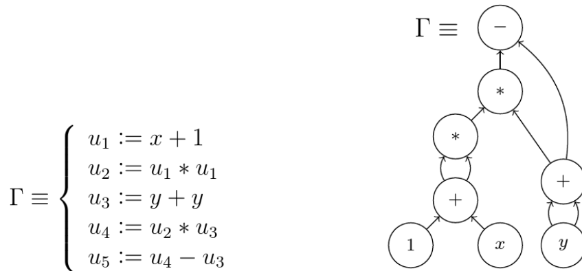
Figure 50. Linear and graph representation of an SLP to evaluate the function 2y(x + 1)^2 - 2y
