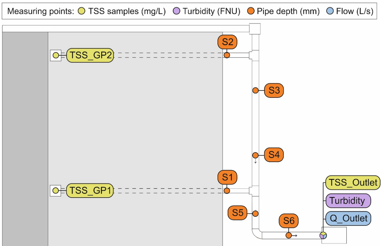
Figure 2. Street section physical model scheme
