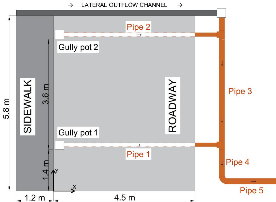
Figure 2. Street section physical model scheme
