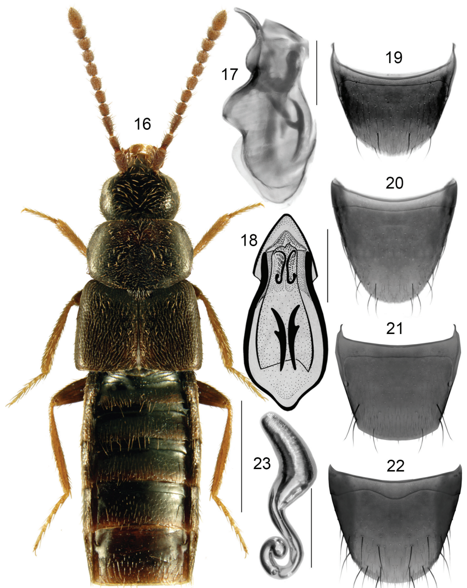
Figures 16–23. Boreophilia islandica (Kraatz): 16 habitus 17 median lobe of aedeagus in lateral view 18 median lobe of aedeagus in dorsal view 19 male tergite VIII 20 male sternite VIII 21 female tergite VIII 22 female sternite VIII 23 spermatheca. Scale bars: 1 mm (habitus); 0.2 mm (remaining).
