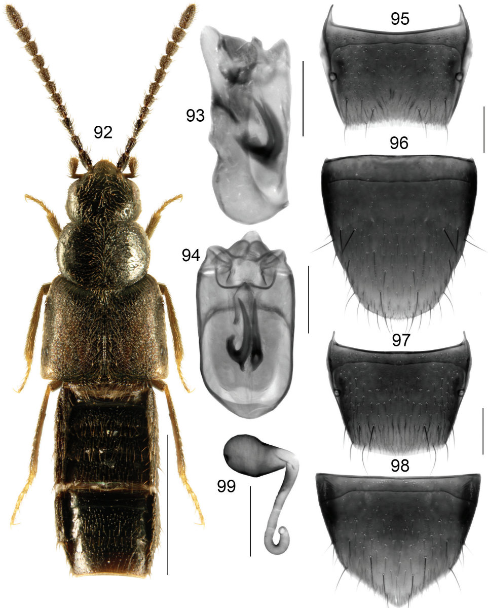
Figures 92–99. Boreophilia subplana (J Sahlberg): 92 habitus 93 median lobe of aedeagus in lateral view 94 median lobe of aedeagus in dorsal view 95 male tergite VIII 96 male sternite VIII 97 female tergite VIII 98 female sternite VIII 99 spermatheca. Scale bars: 1 mm (for habitus); 0.2 mm (remaining).
