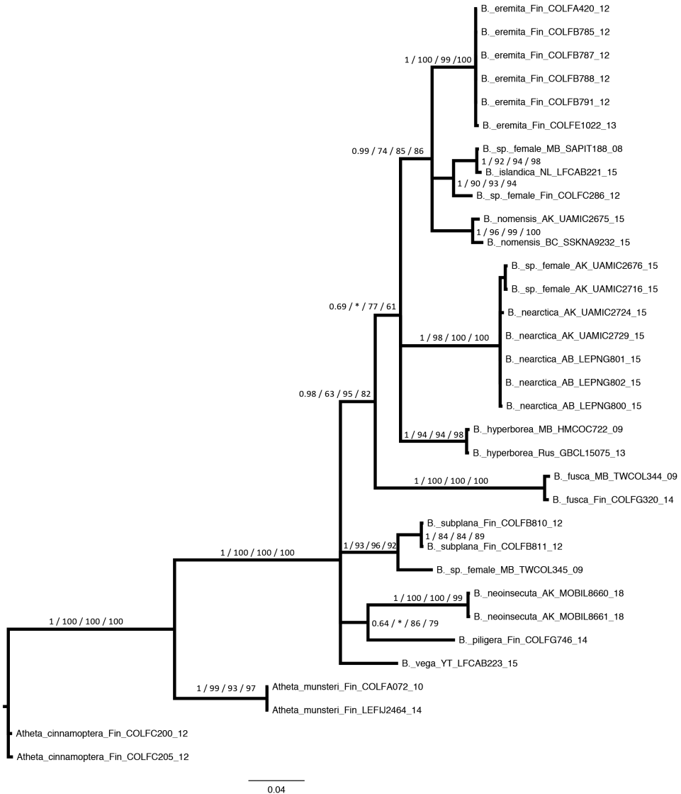
Figure 1. Fifty percent majority rule consensus phylogram from the Bayesian analysis with branch support values provided from left to right as: estimated posterior probabilities, maximum likelihood bootstrap proportions, ultrafast bootstrap values, and an SH-aLRT test values, with * = bootstrap values below 50%. Taxon identity is indicated for each sequence, followed by abbreviations of locality, and BOLD process IDs (see Table 1).
