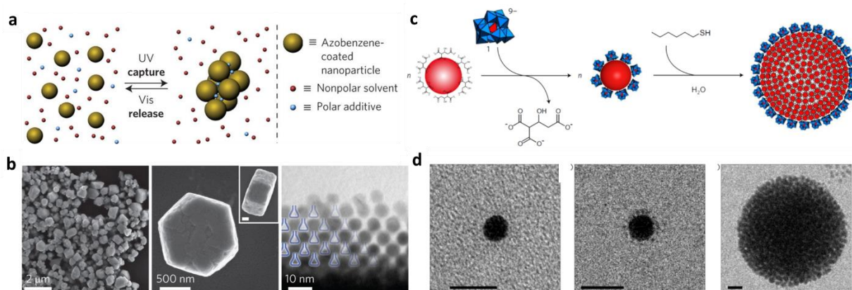
Figure 5. a) Schematic representation of the reversible trapping of molecules during light-induced self-assembly of NPs. b) TEM images (at different magnifications) of colloidal crystals prepared by exposing 6 nm Au NPs to ultraviolet light (scale bar in the inset, 200 nm). Reproduced with permission. [62] Copyright 2016, Nature Publishing Group. c) Synthesis of water-soluble spherical assemblies of 200 nm in diameter using hexanethiol to polyoxometalate-protected Au NPs of 4 nm. d) Cryo-TEM images of the initial citrate-protected Au NPs, the polyoxometalate-protected Au NPs and the 200 nm spherical assemblies. Scale bar, 10 nm. Reproduced with permission. [63] Copyright 2016, Nature Publishing Group.
