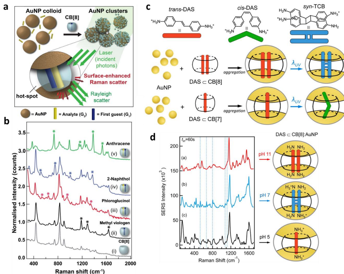
Figure 2. a) Schematic representation of Au NPs aggregation induced by CB[8], which enables SERS detection of polyaromatic hydrocarbons through the formation of a ternary supramolecular complex (b) SERS spectra of CB[8] in the absence (i) and in the presence of different PAHs and a fixed electron deficient guest (5 \mu M). Reproduced with permission. [41] Copyright 2012, American Chemical Society. c) Schematic of diaminostilbene (DAS) photodimerization and photoisomerization in the presence of CB[8] and CB[7], respectively. d) SERS spectra of DAS and the photodimerization product when encapsulated in CB[8] between NPs. Reproduced with permission. [43] Copyright 2013, American Chemical Society.
