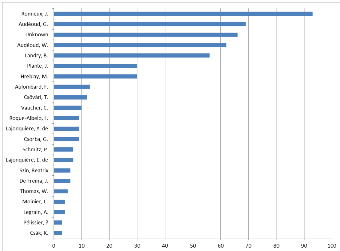
Fig. 5. Primary types of Lepidoptera in the MHNG by collectors (53 in total; shown all with \geq 3 ).
