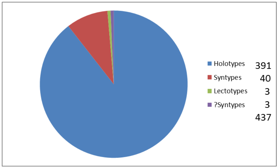
Fig. 1. Primary types of Lepidoptera in the MHNG by type category.
