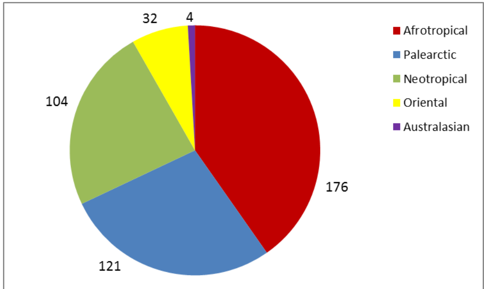
Fig. 3. Primary types of Lepidoptera in the MHNG by geographical realm.
