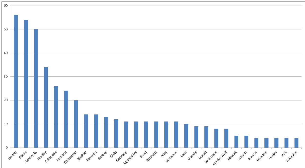
Fig. 4. Primary types of Lepidoptera in the MHNG by authors of taxon descriptions (67 in total; shown all with \geq 4 ).
