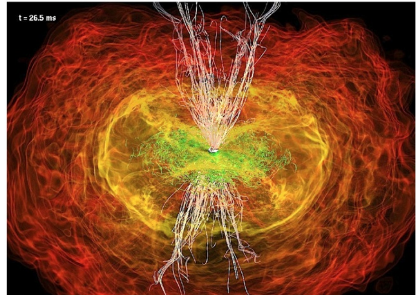
Figure 1. Snapshots at representative times of the evolution of the density, over which the magnetic-field lines are superimposed. The top row shows the evolution from two neutron stars to a black hole ( t = 13.8 ms), while those in the lower row show the evolution of the black hole in the torus and on the equatorial plane, while white lines show the magnetic field. The size of the neutron stars is \sim 90/170 km, while the horizon has a diameter of \sim 30 km. Reports on Progress of Physics arXiv:1607.03540 [gr-qc].
