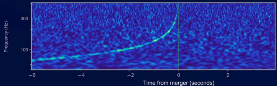
Gravitational-wave strain
