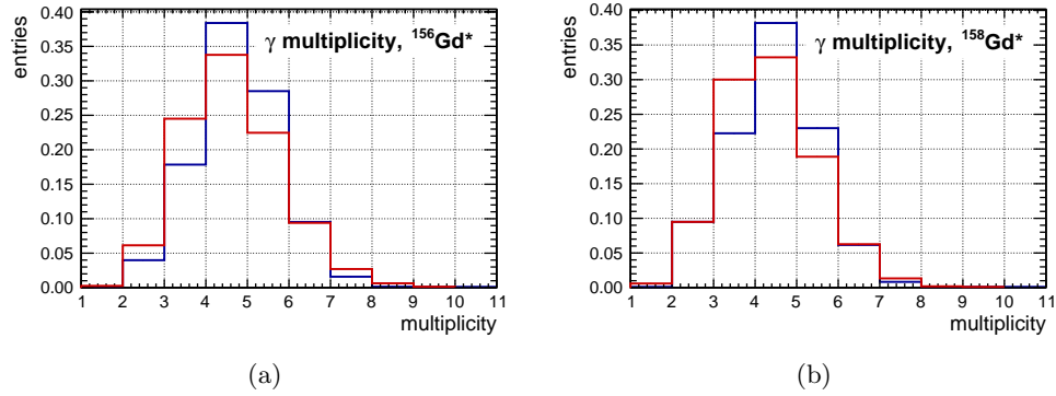
Figure 1: Gamma multiplicity of the deexcitation cascade simulated in GLG4sim (blue) and FIFRELIN (red), for the cascade of the ^{156}\text{Gd} isotope (a) and the ^{158}\text{Gd} (b).
