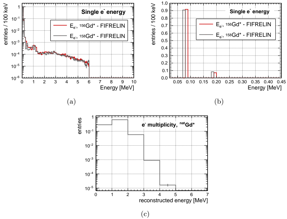
Figure 3: Energy distribution of the electrons from the deexcitation cascade simulated in FIFRELIN (Fig. (a) and (b)), for the cascade of the ^{156}\text{Gd} isotope (red) and the ^{158}\text{Gd} (gray). The multiplicity of electrons per cascade is presented Fig. (c) for natural Gd.
