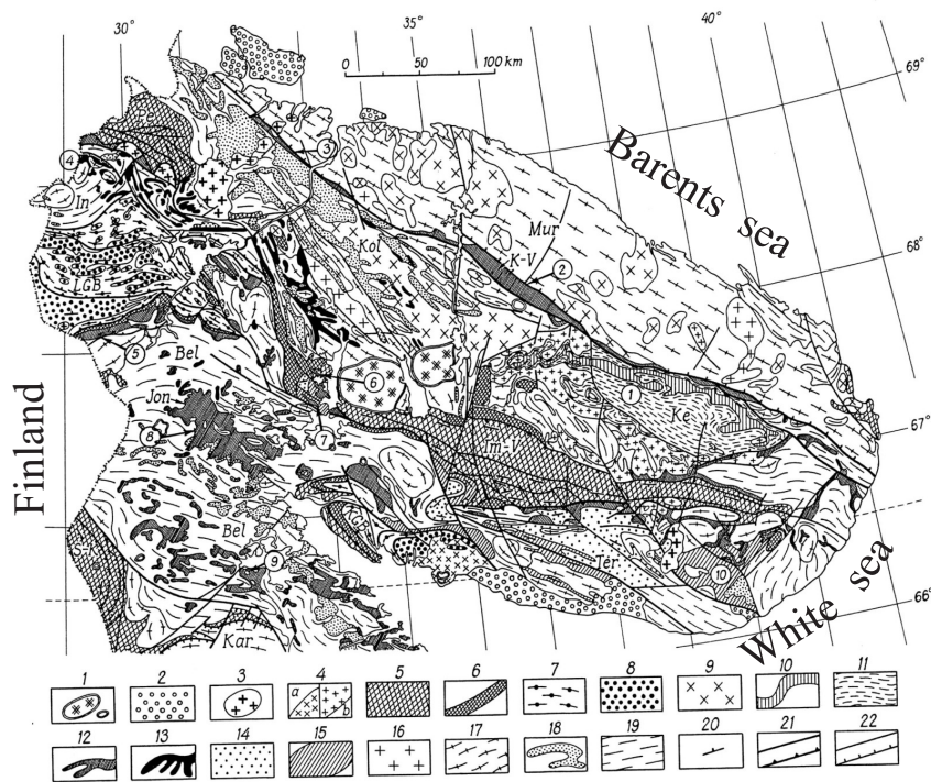
Fig. 1. Geological structural map of the Kola region of the Baltic Shield (from Mitrofanov et al. 1995). Domains: Mur – Murmansk, Kol – Kola, Bel – Belomorian, Ter – Tersky, Ke – Keivy, In – Inary. Belts: Jon – Yona, K-V – Kolmozero-Voronja (Archean greenstone belts); LGB – Lapland, KGB – Kandalaksha-Kolvitsa (granulate belts); Pe – Pechenga, Im-V – Imandra-Varzuga, S-K – North-Karelian (Early Proterozoic rocks); (1) contours of Paleozoic intrusions (a-nepheline syenite, b-ultramafic alkaline rocks); (2) Upper Proterozoic sedimentary rocks. Early Proterozoic: (3) granite, granodiorite and diorite; (4) charnokite and granite (a), alkalinegranite (b); (5) volcanic-sedimentary rocks; (6) anorthosite and gabbro-anorthosite (in Keivy – Archean), gabbro, pyroxenite, peridotite. Early Proterozoic (or Archean?): (7) basic and intermediate granulite; (8) acid granulite. Late Archean: (9) granodiorite, diorite and enderbite; (10) alumina and super-alumina gneiss and schist; (11) acid gneiss; (12) fragments of greenstone belts (gneiss, amphibolites and komatiite); (13) fragments of banded iron formation (gneiss, amphibolites and ferruginous quartzite); (14) gneiss and schist; (15) gneiss and amphibolites; (16) granodiorite and diorite; (17) plagiogranite and granite-gneiss; (18) kyanite-garnet-biotite gneiss; (19) granite-gneiss, gneiss, migmatites and, rarely, amphibolites. (20) strike and dip; (21) subvertical faults and gentry dipping thrusts that separate the Proterozoic domains; (22) subvertical faults and thrusts. Encircled numbers indicate type-sections: 1 – Keivy, 2 – Kolmozero, 3 – Ura-Guba, 4 – Kaskama, 5 – Korva, 6 – Ar-Varench, 7 – Voche-Lambina, 8 – Iona, 9 – Kovdozero, 10 – Tersky
