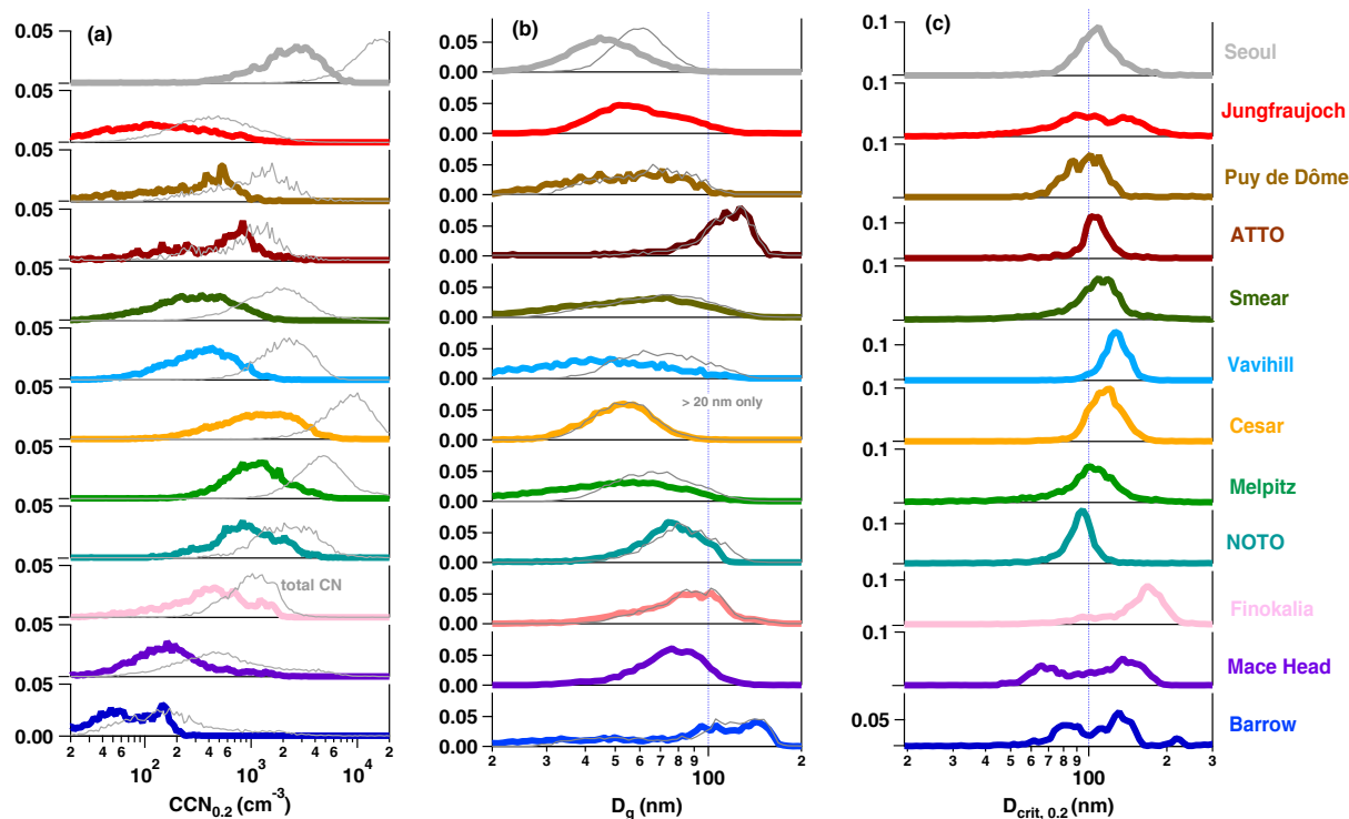
Figure 3. (a) Normalised frequency distributions of CCN number concentration at SS = 0.2\% and total particle number in light grey, (b) geometric mean diameter D_g , and (c) critical diameter D_{crit} at SS = 0.2\% . The grey lines in (b) are based on size distributions starting at 20 nm. The critical diameter is derived from the total CCN concentration ( SS = 0.2\% ) and the integrated particle number concentration starting from the largest diameter (see Sect. 2.2.2 for details). Note that seasons are not represented by an equal number of data points at each station which can lead to small biases in the frequency distributions. In (a) and (c) all axes start at 0.00.
