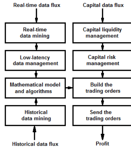
Fig. 4 Data logical scheme of automated trading system
