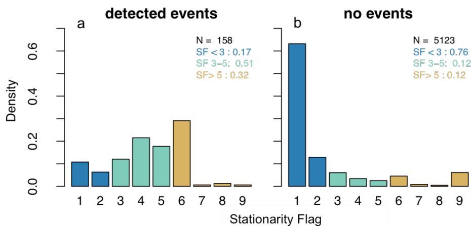
15 Figure 3: Stationarity flag frequency distribution of half-hourly timestamps, separating between fluxes that were influenced by events (a) and those where no events were detected (b). Stationarity flags were grouped into the three classes high (dark blue), medium (light blue) and low (light brown) stationarity. The total count of timestamps is slightly above the sum of timestamps available during the study period (5280) due to an occasional occurrence of several events in a single half-hour window.
