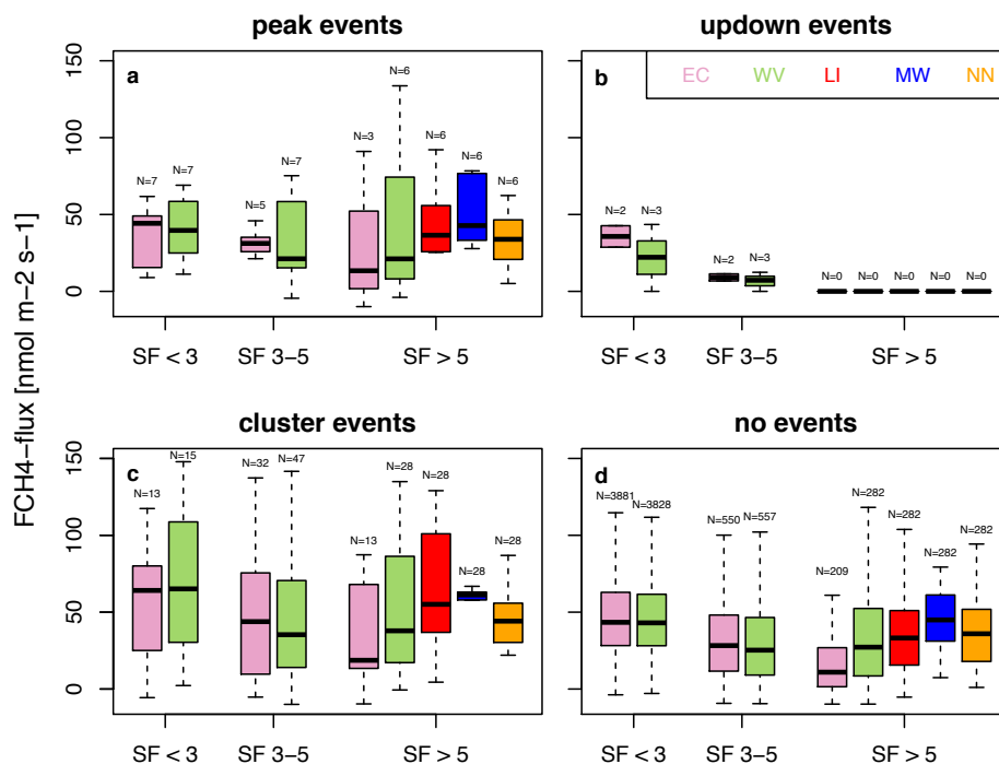
Figure 4: Methane fluxes based on the EC (purple) and wavelet (green) flux processing method for three stationarity flag (SF) categories during different event types at tower 2. For SF > 5, where methane fluxes based on the EC method would be excluded during the regular post-processing quality control, in addition the values for the three gapfilling methods (red: LI; blue: MW; orange: NN) are shown. For details on graph features, please refer to Figure 2.
