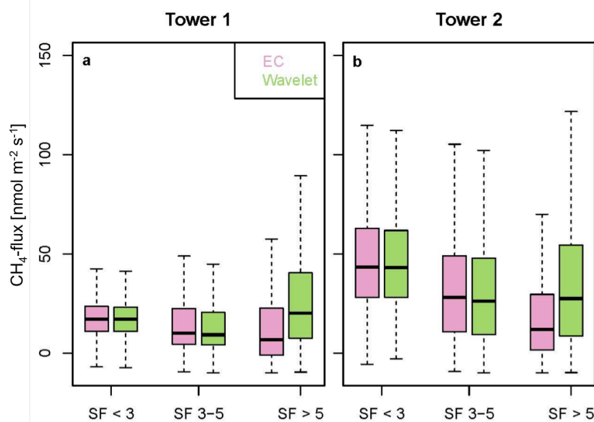
Figure 1: Median and variability of non-gapped methane fluxes based on the EC (purple) and wavelet (green) flux processing methods for different stationarity classes at towers 1 (a) and tower 2 (b). Black horizontal bars give the median, colored boxes indicate the interquartile range covered by the 2 nd and 3 rd quartile, while whiskers show the minimum and maximum, respectively, flux rates.
