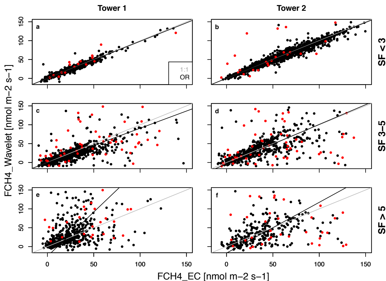
5 Figure A3: Impact of events on the direct intercomparison of half-hourly flux rates between wavelet and eddy-covariance processing methods, sorted by tower and stationarity flag (SF) category. The displayed dataset includes gapfilled data, where linear interpolation was used to fill gaps for the EC method under low stationarity. Fluxes influenced by events are plotted in red, while 'no events' cases are black. The thin grey line gives the 1:1 line, the black line the fit of the orthogonal regression (OR) analysis.
