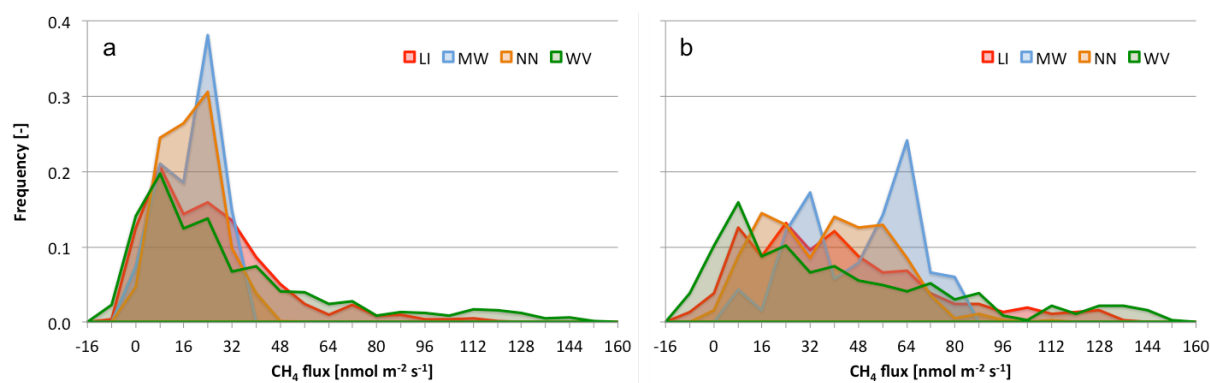
15 Figure 2: Frequency distribution of flux rates (a: tower 1; b: tower 2) produced by the three gapfilling approaches (red: linear interpolation (LI); blue: moving window (MW); orange: neural network (NN)), compared against the reference flux values derived from the wavelet raw data processing method (WV, green).
