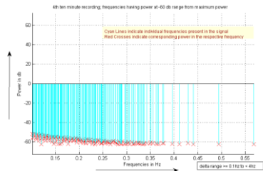
Fig. 34 Delta Range frequencies present at -60 db threshold in the Divine Omdasji Sound Meditation recording of the fourth ten minutes
