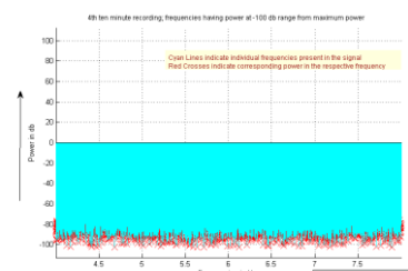
Fig. 39 Theta Range frequencies present at -100 db threshold in the Divine Omdasji Sound Meditation recording of the fourth ten minutes
