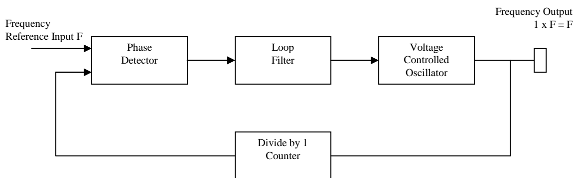
Fig 82. Block Diagram of a Phase Locked Loop (Courtesy: www.cardinalxstal.com/docs/notes/cardinal_phase_lock_loop_basics.pdf , as on Feb 28, 2007)
