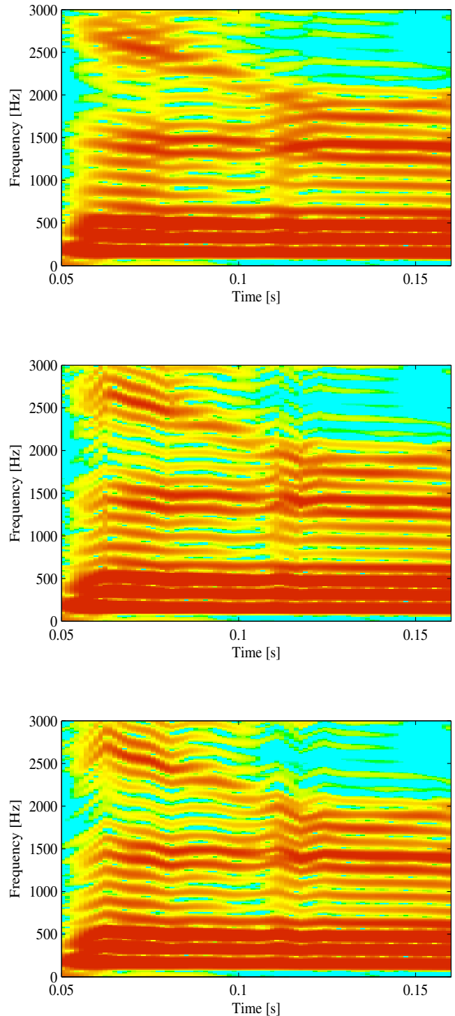
Fig. 2. Spectrograms produced by DFT, FChT and aDFT depicted in the first, second and third row, respectively.
