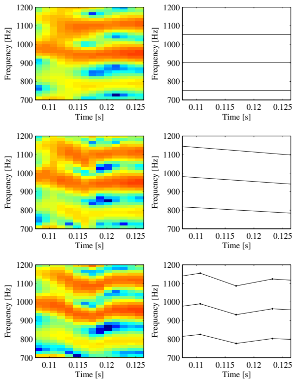
Fig. 1. Three different transforms and their respective frequency bases for a single analysis window. First row depicts the spectrogram and frequency basis of the central frame of DFT, second row of FChT and third row of aDFT.
