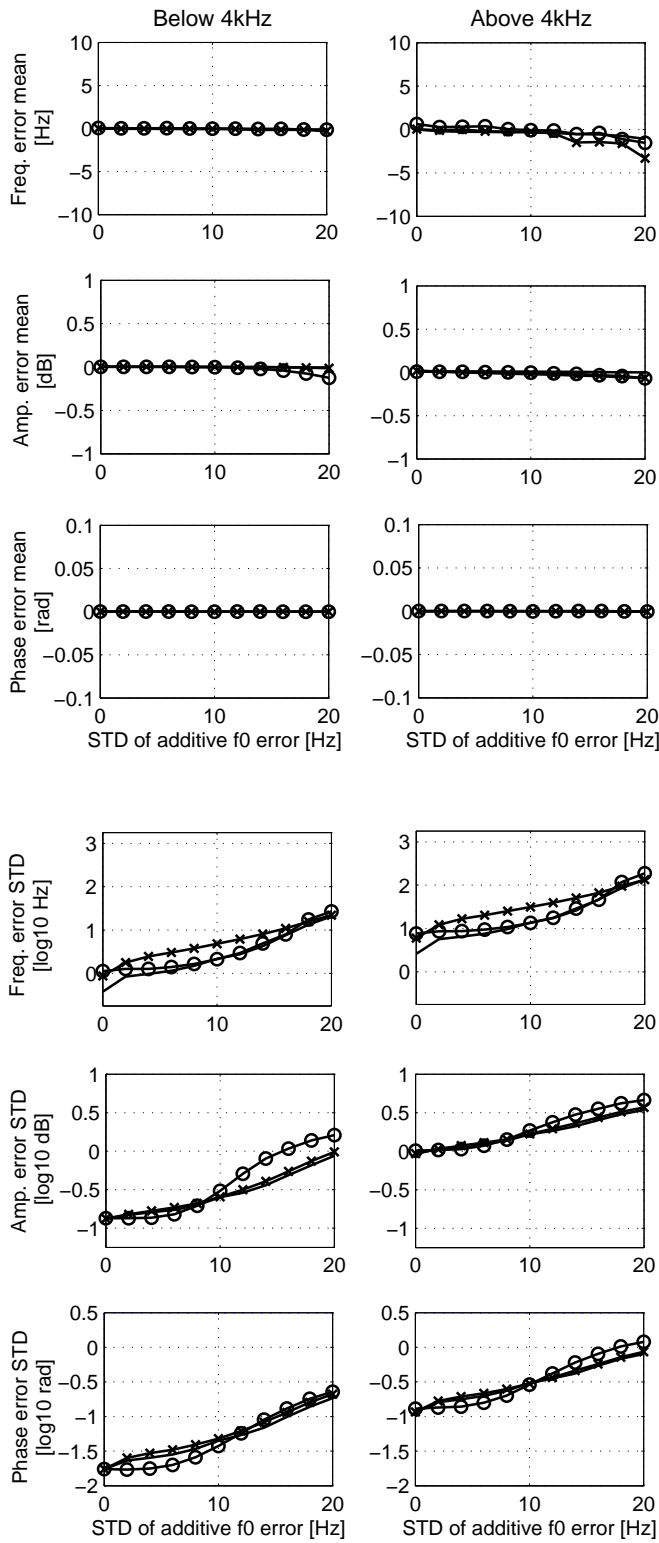
Fig. 5. Error of sinusoidal parameters with respect to a potential error on the f_0 curve provided to the analysis methods, comparing full adaptivity with linear adaptivity during the f_0 refinement steps.
