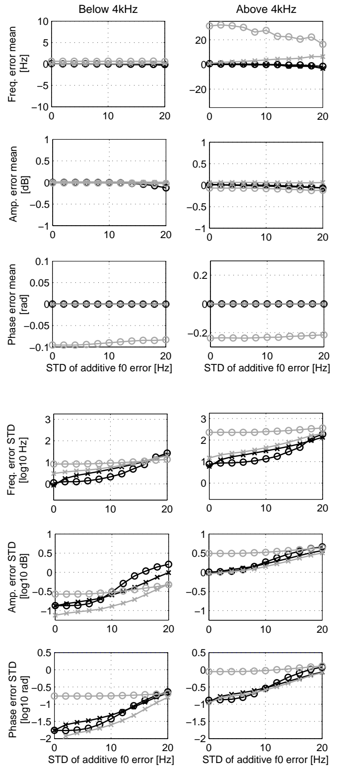
Fig. 6. Error of sinusoidal parameters with respect to a potential error on the f_0 curve provided to the analysis methods, comparing LS solution with Peak Picking in the last analysis step.
