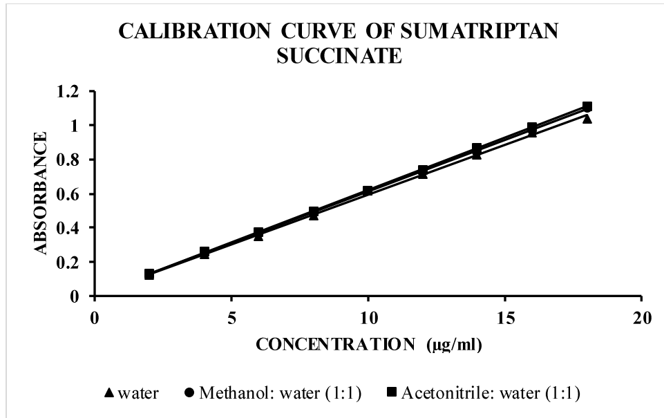
Fig.2: Calibration curves of Sumatriptan succinate
