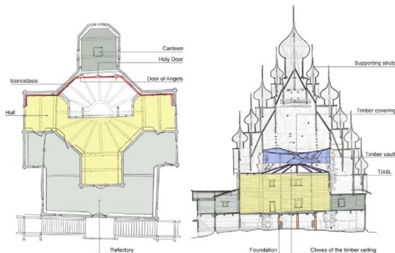
Fig.8 Scheme related to the architectural composition of the Church of the Transfiguration on Kizhi Island. Thanks to the historic previous documentation it has been possible to understand and know about the original composition of the building. Which where the main elements and how they were located in the structure
