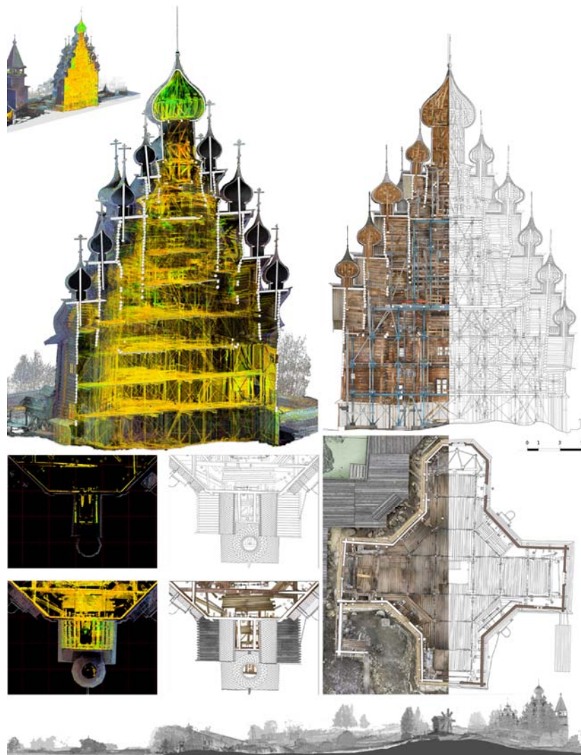
Fig.14 Different phases of the reprocessing data for the digital survey of the Pogost Complex on Kizhi Island, Russia. For this projects, the post production has involved accurate elaboration of technical drawings for the representation and comprehension of traditional timber technologies and architectural aspects
