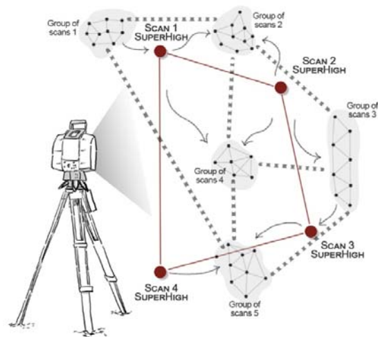
Fig.11 In the organization of wide digital survey, it could be useful to use different levels of resolution for performing the scan words defining specific polygonals. In this image Scans 1, 2, 3, 4 have “super high” resolution and they create a close polygonal loop. On this basis, the other scans registered in smaller groups, can be linked and find a correct mutual position. By registering each group of scans with the main polygonal of super high scan words, each group will be definitely also correctly linked with the other groups of scans
