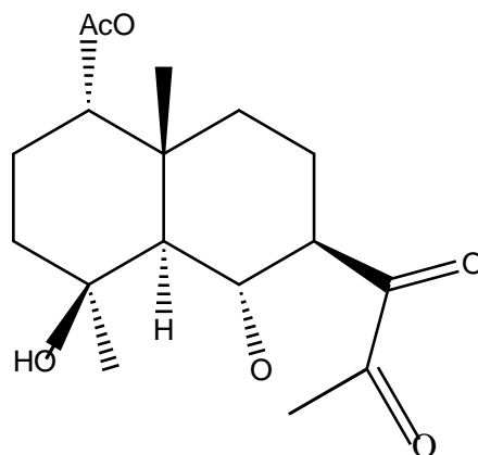
Figure 12: structure of 4-epi-1 \alpha -acetoxymarbusculin A.
