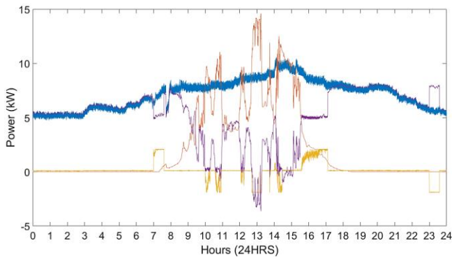
Figure 4. Power measurements of UCY load (blue), PV production (orange), battery demand (yellow) and net load (grid power) (purple).
