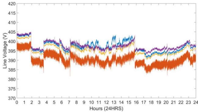
Figure 5. Voltage levels of the PV (blue), the battery (orange), the PCC (yellow) and the grid (purple).
