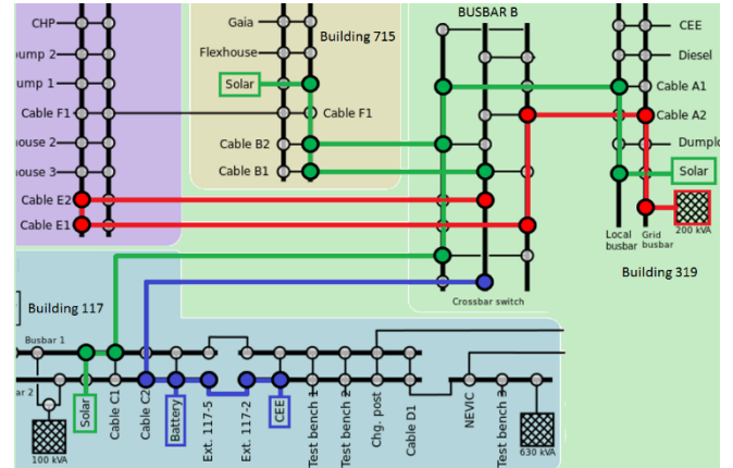
Figure 3. Diagram of the actual experimental setup at SYSLAB showing the switchboard connections. The PCC is replicated by Busbar B.
