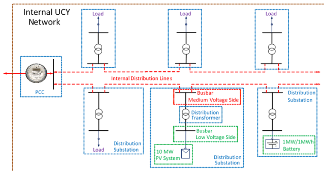
Figure 1. The envisaged UCY \mu G connection diagram.
