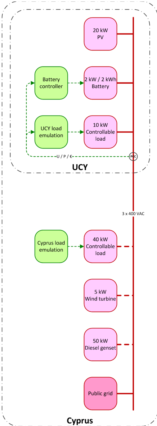
Figure 2. Diagram of the experimental setup at SYSLAB.
