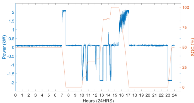
Figure 6. Power demand (blue) and SOC (orange) of the battery.
