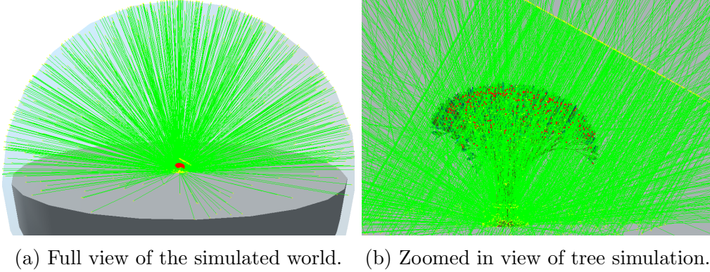
Figure 3: Shown are two example views of the full simulated world containing a single tree. The full view of the simulated scene displays the distribution of simulated diffuse light (green lines) starting on the sky-dome. The zoomed in view displays the tree and registered hits on leaves (red dots) as well as the simulated direct normal irradiance source defined as disc source at the location of the Sun, illuminating the entire tree.
