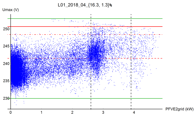
Fig. 19. Net PV production with smart energy storage – PV 5.2 kWp
