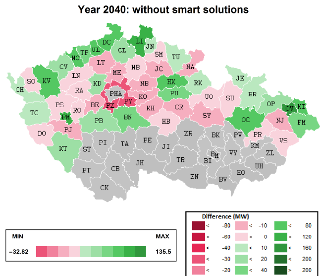
Fig. 1. Expected lack of DER hosting capacity in LV grids in 2040 in case that smart grid solutions are not implemented
