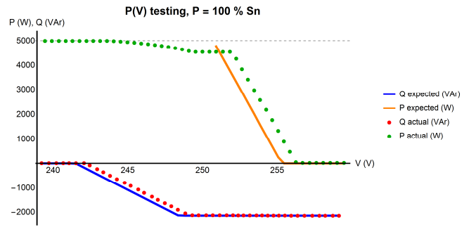
Fig. 8. P (V) function lab test results for Fronius PV inverter
