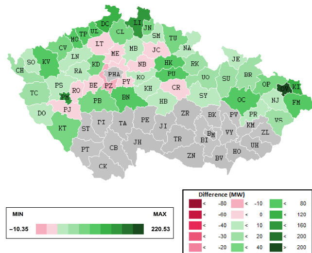
Fig. 20. Expected lack of DER hosting capacity in LV grids in 2040 in case that smart grid solutions are implemented
