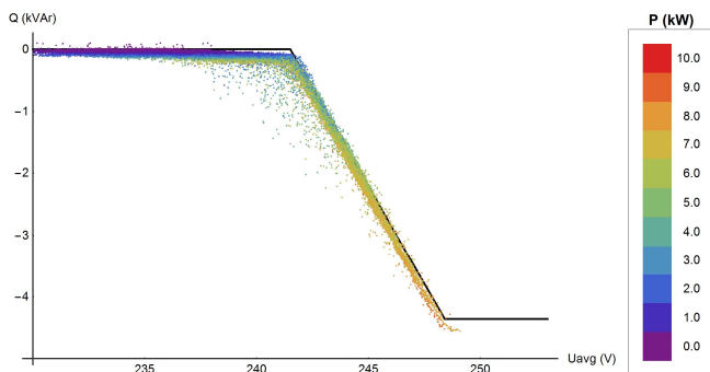
Fig. 11. Smart PV inverter operation points in April 2018
