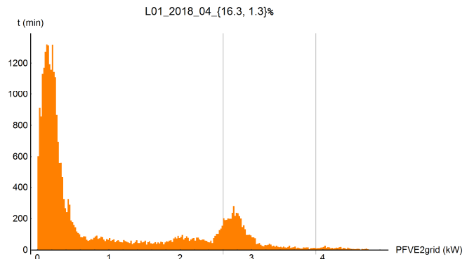
Fig. 17. Net PV production with smart energy storage – PV 5.2 kWp
