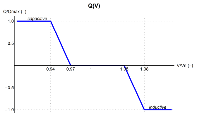
Fig. 4. Autonomous Q (V) function of smart PV inverter
