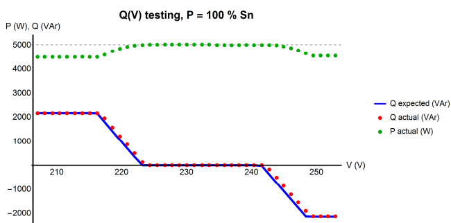
Fig. 7. Q (V) function lab test results for Fronius PV inverter
