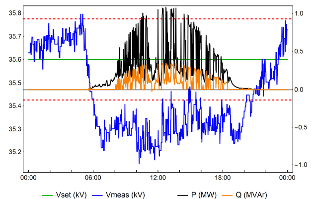
Fig. 13. Demonstration of volt-var control system on 1.1 MWp PV
