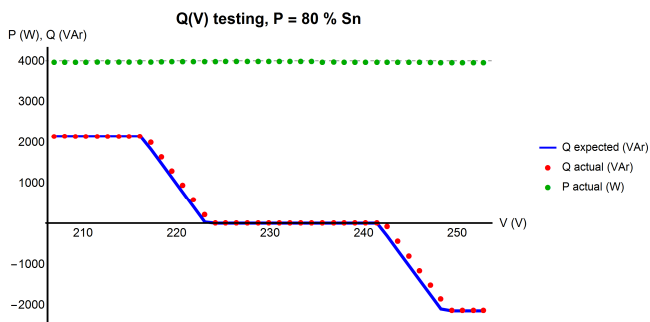
Fig. 6. Q (V) function lab test results for Fronius PV inverter
