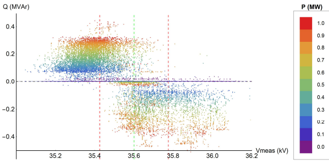
Fig. 14. Long-term statistical assessment of volt-var control system behavior on PV Zamberk (installed capacity 1.1 MWp)
