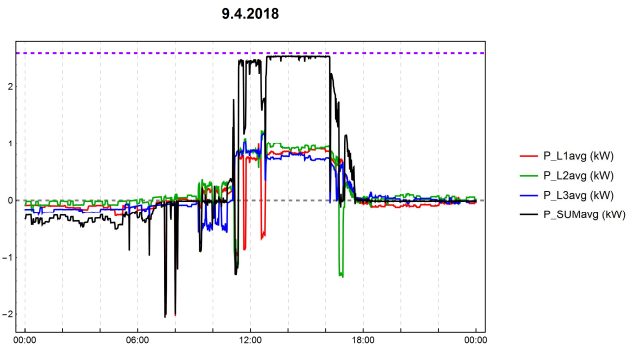
Fig. 16. Daily behavior of customer with PV and energy storage – PV 5.2 kWp, feed in power limited to 50 % (2.6 kW)
