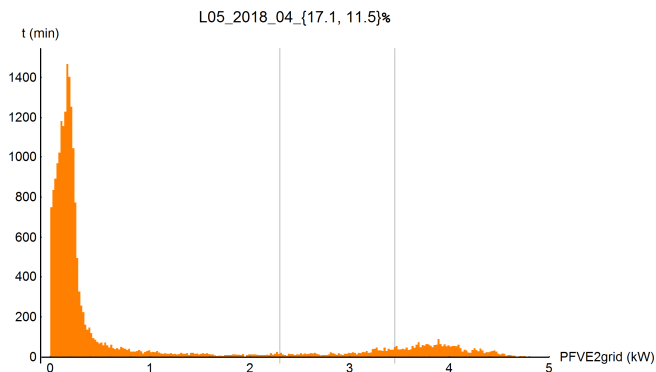
Fig. 18. Net PV production without any energy storage – PV 4.6 kWp
