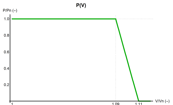
Fig. 5. Autonomous P (V) function of smart PV inverter
