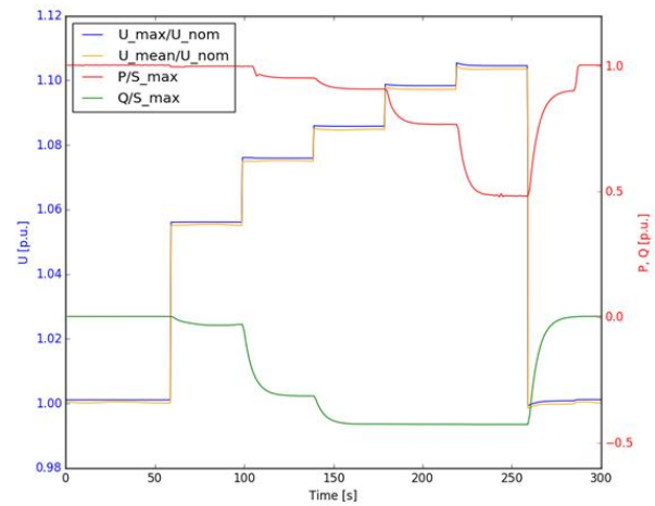
Fig. 9. Control dynamic behavior for Fronius PV inverter
