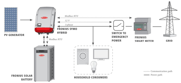
Fig. 15. Fronius solution with smart energy storage
