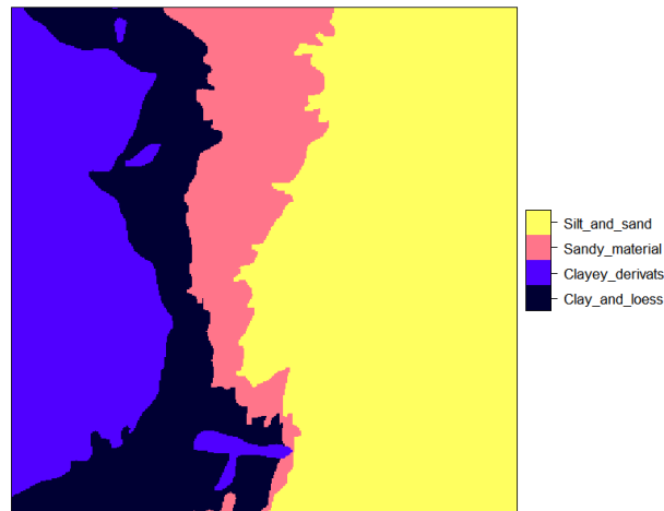
Fig. 4.3 Ebergetzen zones rasterized to 25 m resolution and with correct factor labels.
