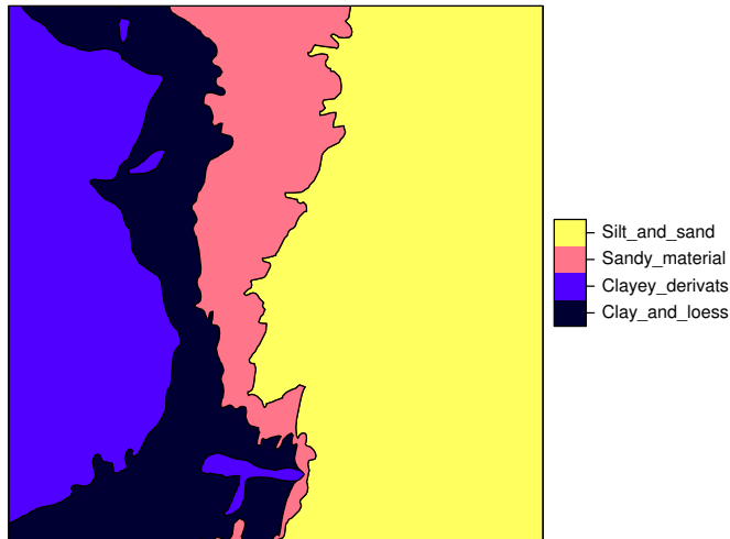
Fig. 4.1 Ebergetzen parent material polygon map with legend.
