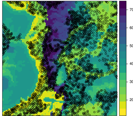
Fig. 6.4 Predicted sand content based on deep learning.
