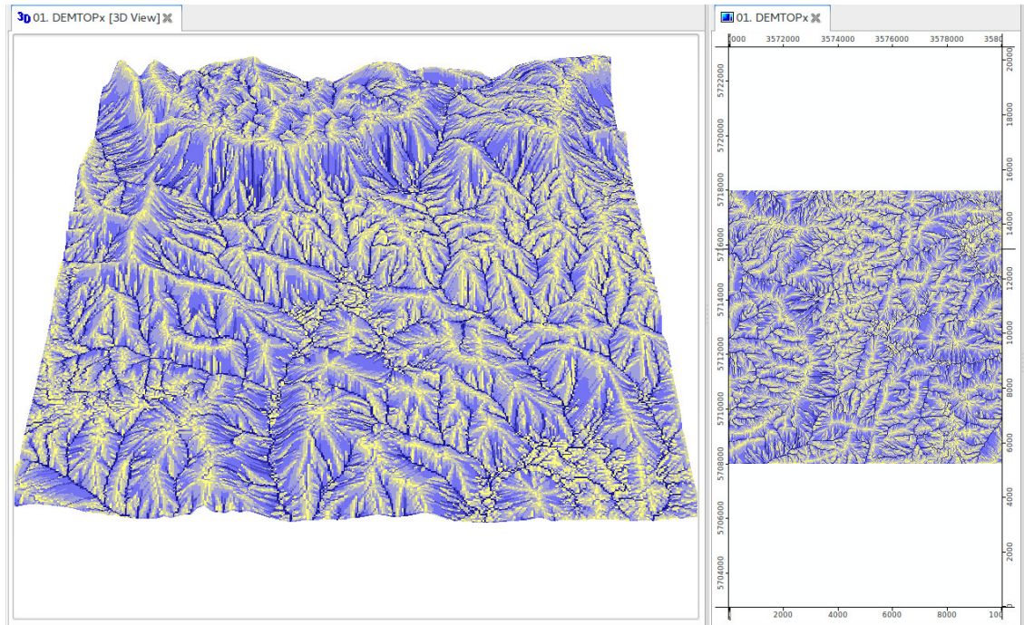
Fig. 2.3 Hydrological flow accumulation map based on the Ebergotzen DEM derived using WhiteboxTools.
