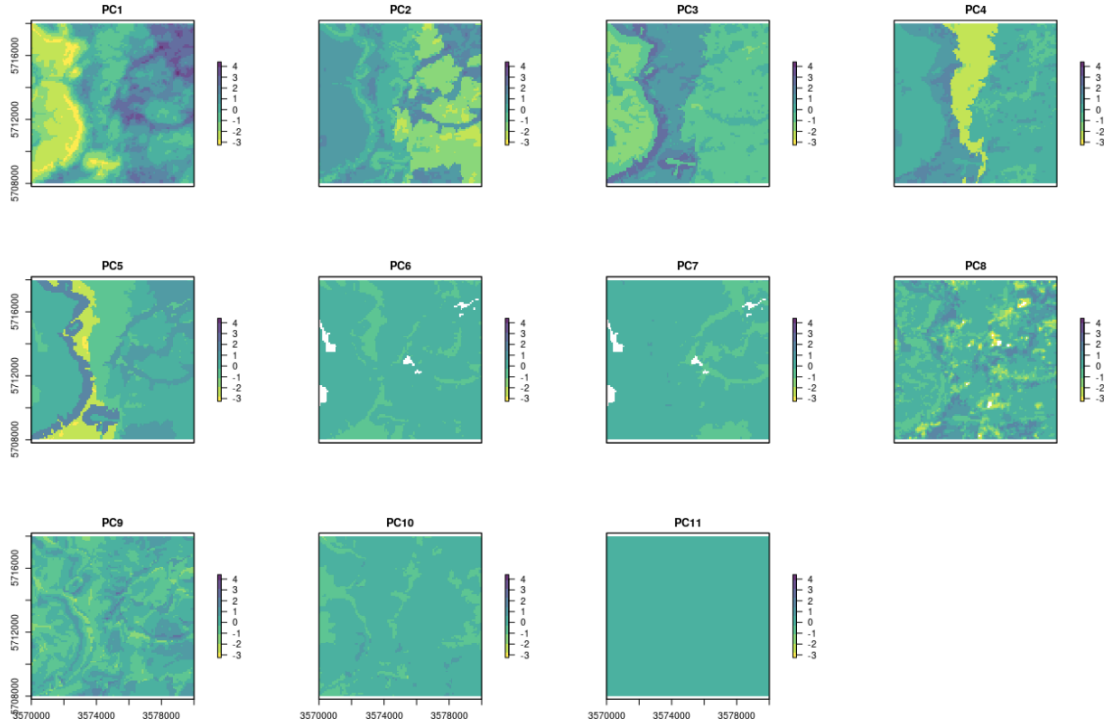
Fig. 4.7 11 PCs derived using input Ebergetzen covariates.
