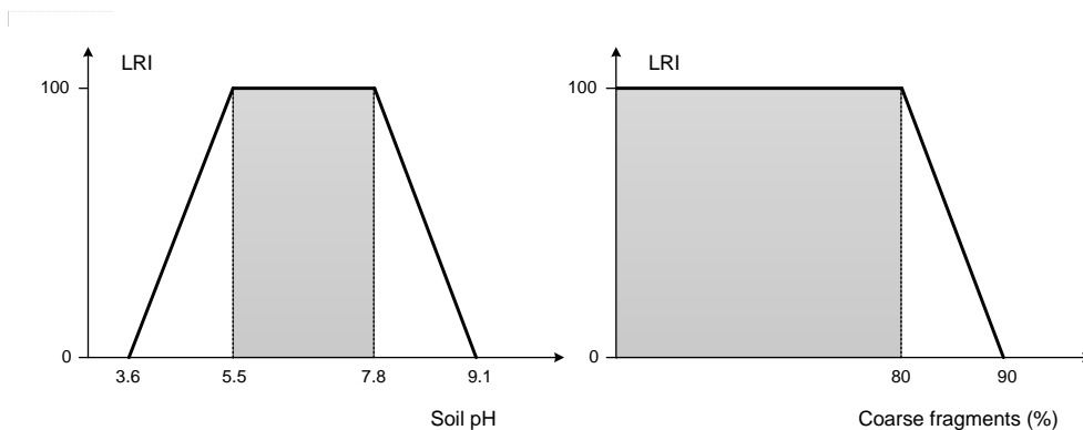
Fig. 3.5 Derivation of the Limiting Rooting Index: (left) soil pH values and corresponding LRI, (right) coarse fragments and corresponding LRI. Based on Leenaars et al. (2018) doi: 10.1016/j.geoderma.2018.02.046.
