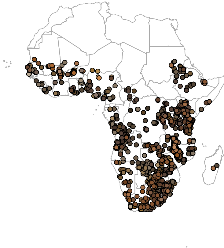
Fig. 3.23 Actual observed soil colors (moist) for the top soil based on the Africa Soil Profiles Database.
