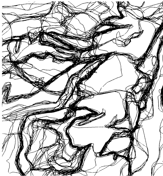
Fig. 1.14 20 photo-interpretations done independently using the same aerial photograph overlaid on top of each other. This illustrates uncertainty of position of soil borders due to operator's subjective concepts. Image credit: Legros (1997).
