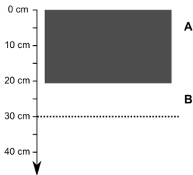
(c) Standard mineral soil profile (missing values)
