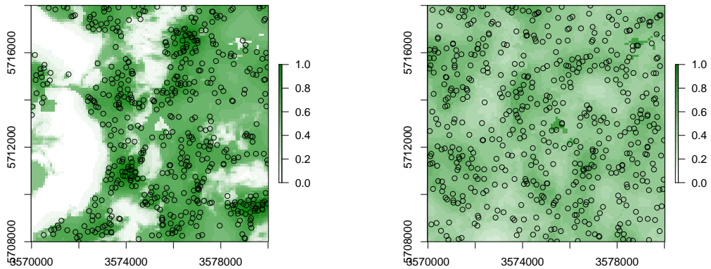
Fig. 5.4 Occurrence probabilities derived for the actual sampling locations (left), and for a purely random sample design with exactly the same number of points (right). Probabilities derived using the ‘ spsample.prob ’ function from the GSIF package. The shaded area on the left indicates which areas (in the environmental space) have been systematically represented, while the white colour indicates areas which have been systematically omitted (and which is not by chance).
