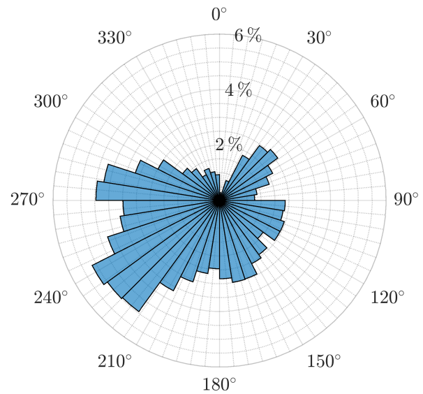
Figure 5. Wind rose of 1 Hz measurement data recorded at a met. mast in Brusow, north-eastern Germany.
