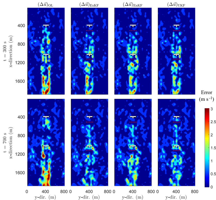
Figure 4. Comparison of absolute values of the estimation errors (in long. flow fields) for state-only estimation with the ExKF, EnKF and UKF at t = 300 s and t = 700 s, with (\Delta \mathbf{u}) = |\mathbf{u} - \mathbf{u}_{\text{SOWFA}}| . The model and KF settings are depicted in Tables 1, 2, and 3. Wind is coming in from the top, flowing towards the bottom. The measured states are depicted by red dots in the flow, not to be confused with estimation error. The KFs consistently improve the instantaneous flow field estimations, noticeably nearby the measurements.
