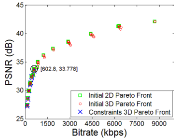
(c) 3D → 2D Pareto front of PSNR vs Bitrate
