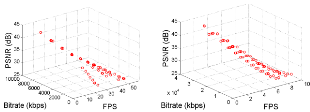
(a) Pareto front of emergency scenery video of Fig. 1(a).
