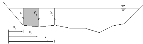
Figure 2: Cross sectional area of the river.
