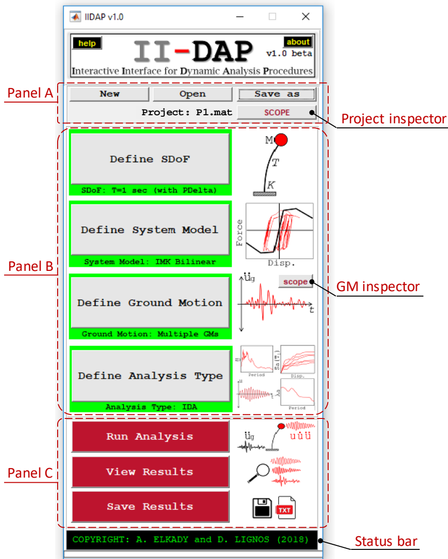
Figure 1. IIDAP v1.0 main console
