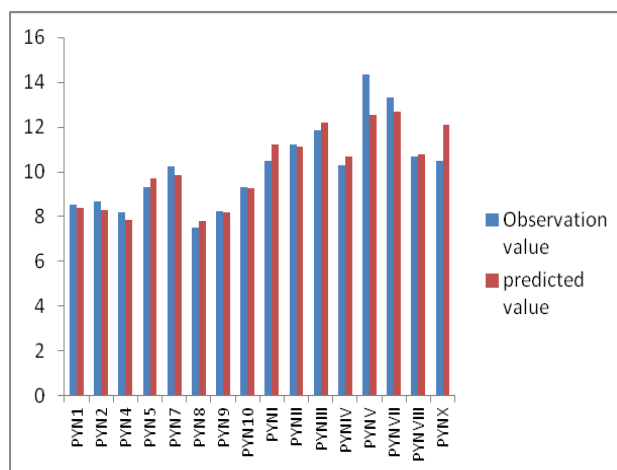
Figure1. Chart of comparison between observed and predicted zone of inhibition for training set.
