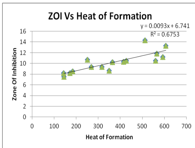
Figure4. Chart of comparison between parameter(heat of formation) and zone of inhibition values for training set.
