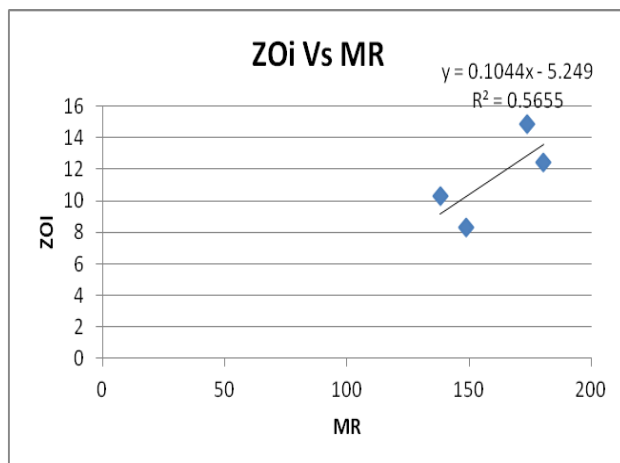
Figure7. Chart of comparison between parameter (MR) andzone of inhibition values for test set.
