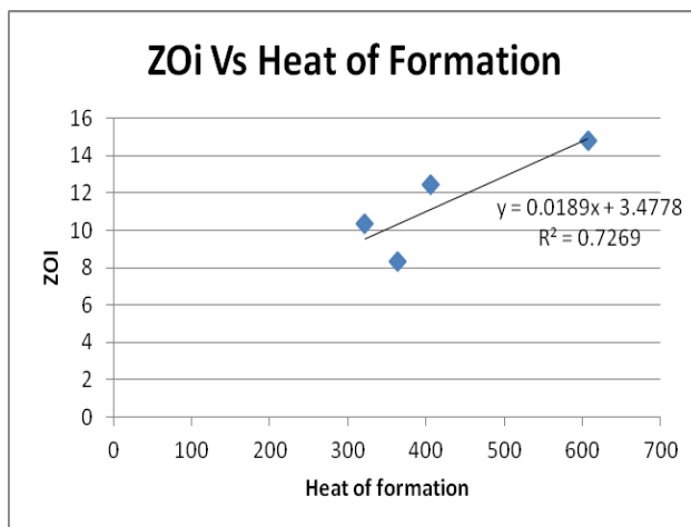
Figure 8. Chart of comparison between parameter (heat of Formation) and zone of inhibition values for r test set.
