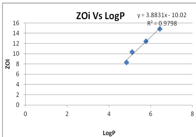
Figure6. Chart of comparison between parameter (Log P) andzone of inhibition values for test set.
