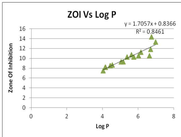
Figure2. Chart of comparison between parameter (Log P) and zone of inhibition values for training set.
