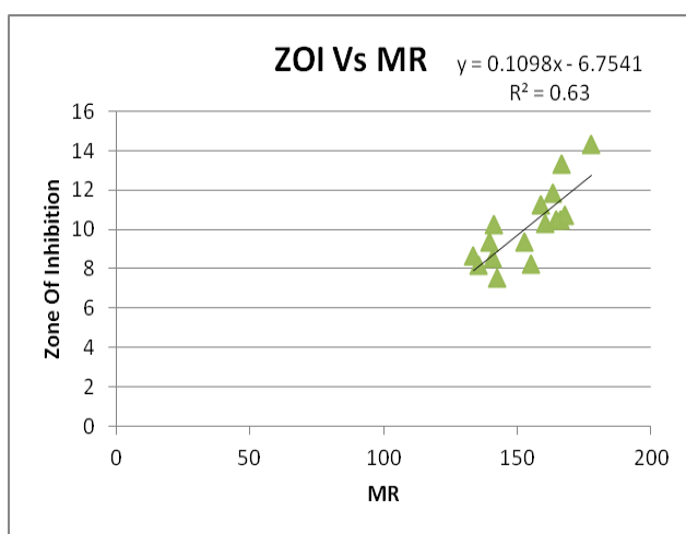
Figure3. Chart of comparison between parameter(Molar refraction) and zone of inhibition values for training set.
