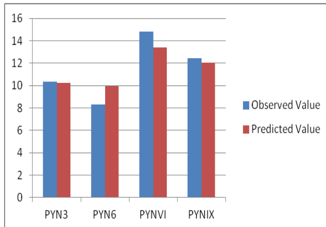
Figure5. Chart of comparison between observed and predicted zone of inhibition value for test set.
