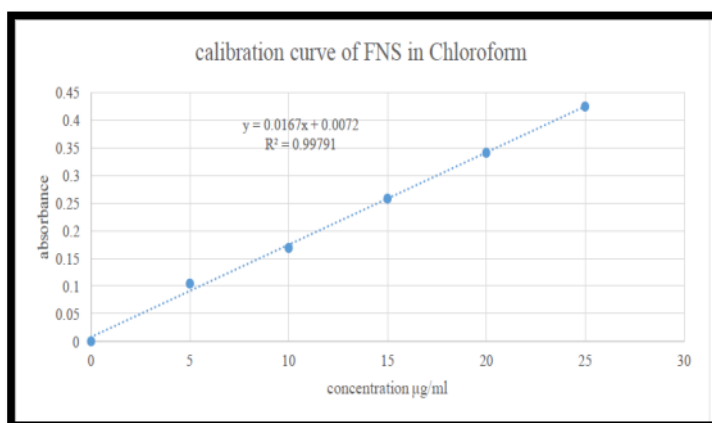
Figure 3. Calibration curve of finasteride.
