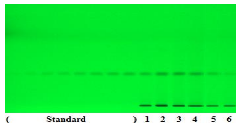
Figure 4. HPTLC Chromatogram of standard Caffeine and AE of different coffee grades.
