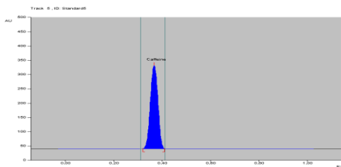
Figure 3. HPTLC Chromatogram of standard Caffeine.
