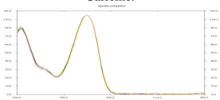
Figure 5. Overlaid UV absorption spectra of standard caffeine and different grades of coffee.
