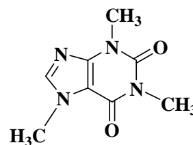
Fig. 1. Chemical structure of Caffeine.
