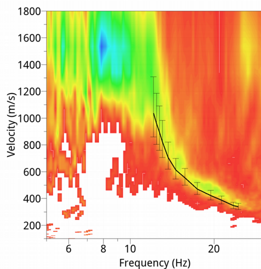
Figure 11: Stacked spectrum from passive measurements. The picked dispersion is also shown as black curve.
