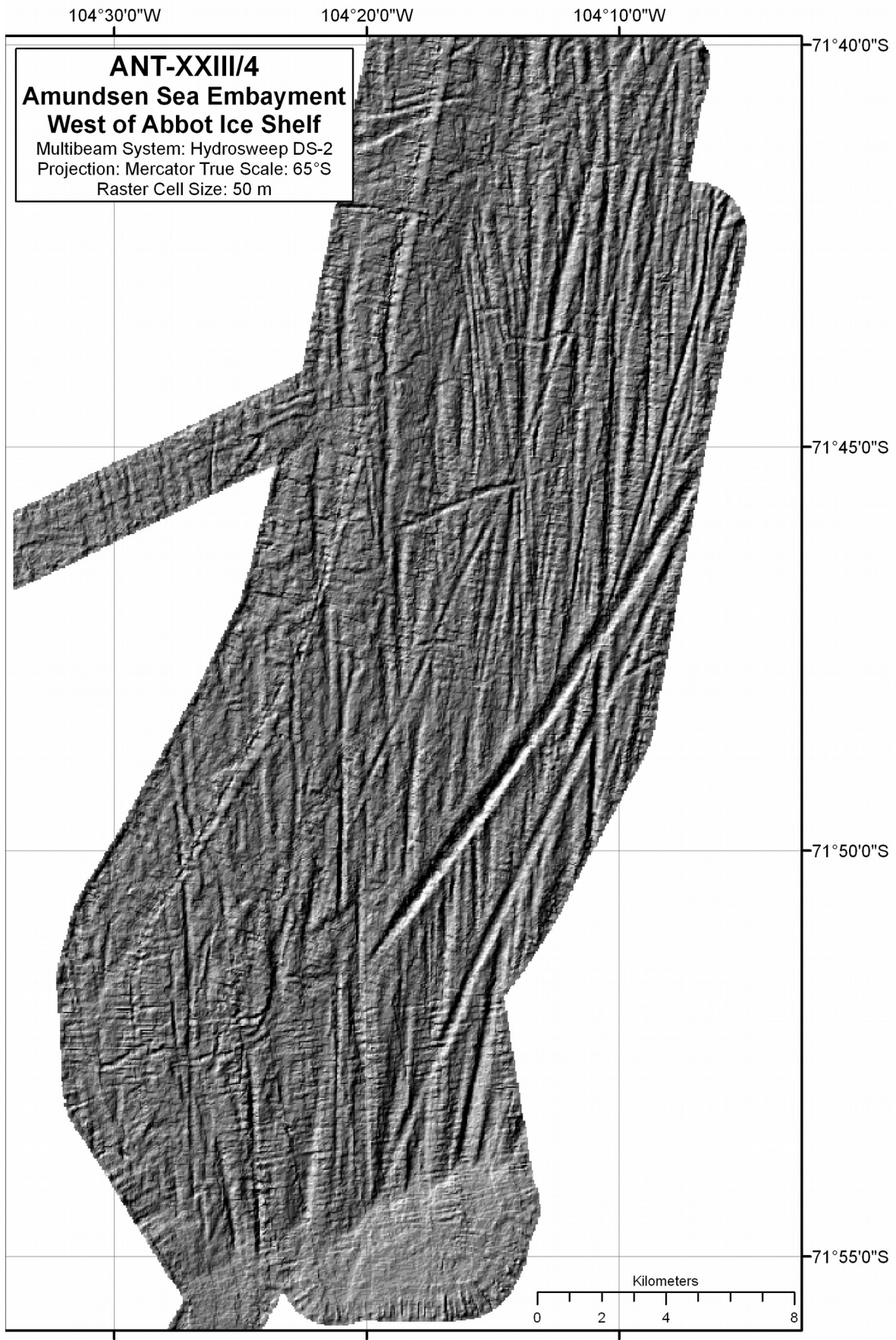
Fig. 1: Hillshade of the survey area west of the Abbot Ice Shelf
