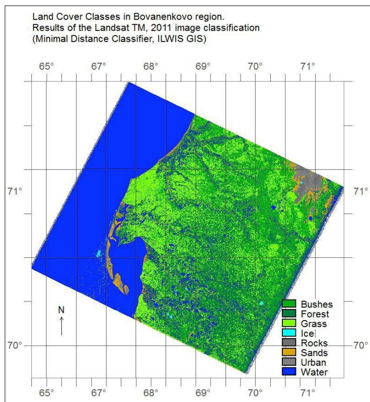
Figure 3. Land Cover Classes: year 2011 (Landsat TM)
