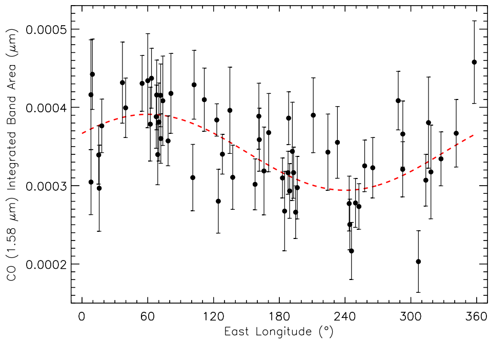
Figure 5: Integrated band area of the 1.58 \mu\text{m} \text{CO} band plotted against sub-observer longitude. The dashed line is a robust sinusoidal fit to the points. The phase difference between the 1.58 \mu\text{m} and 2.35 \mu\text{m} \text{CO} bands is 5 \pm 5^\circ .
