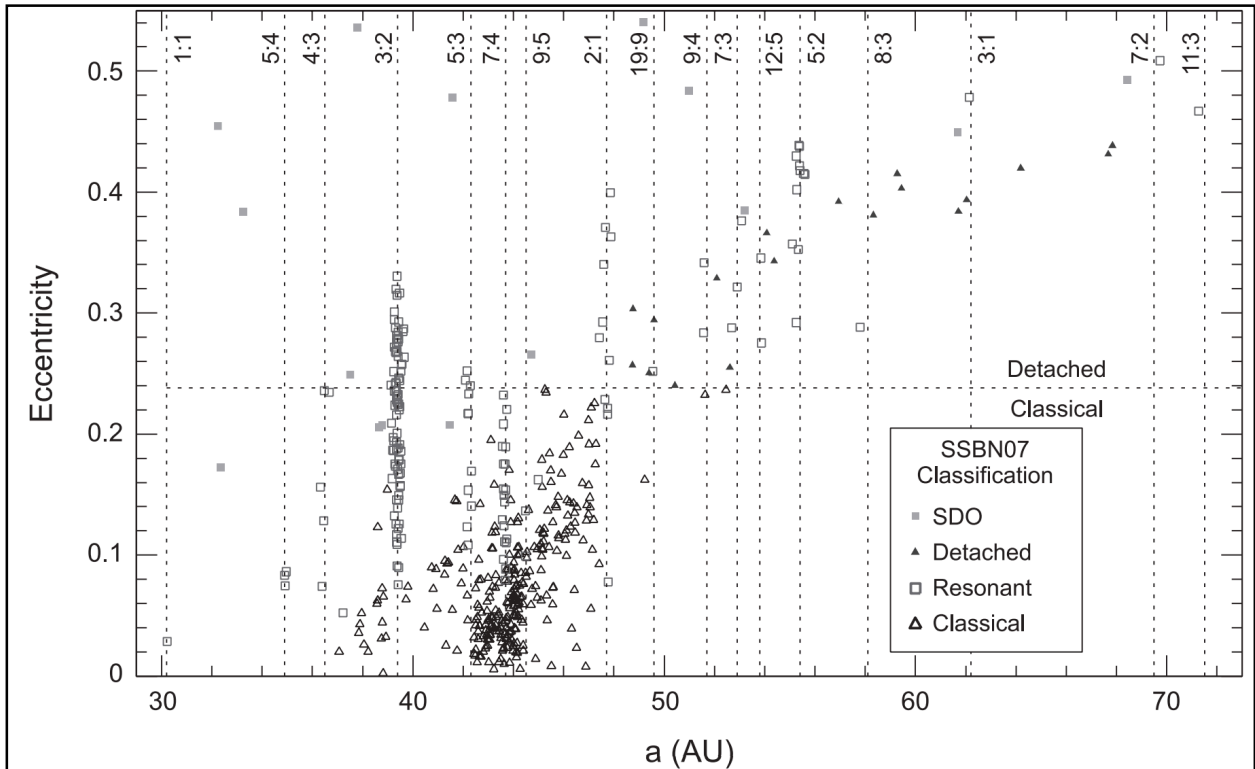
Figure 3: Eccentricity as a function of semi-major axis ( a ) for all KBOs with semi-major axes between \sim 30 and \sim 73 AU known in 2007. The classical definition of the Kuiper Belt is between the 3:2 and 2:1 Neptune resonances (note the higher concentration of objects). Detached objects have semi-major axes beyond the 2:1 resonance and eccentricities greater than 0.24. (From Gladman et al. (2008))
