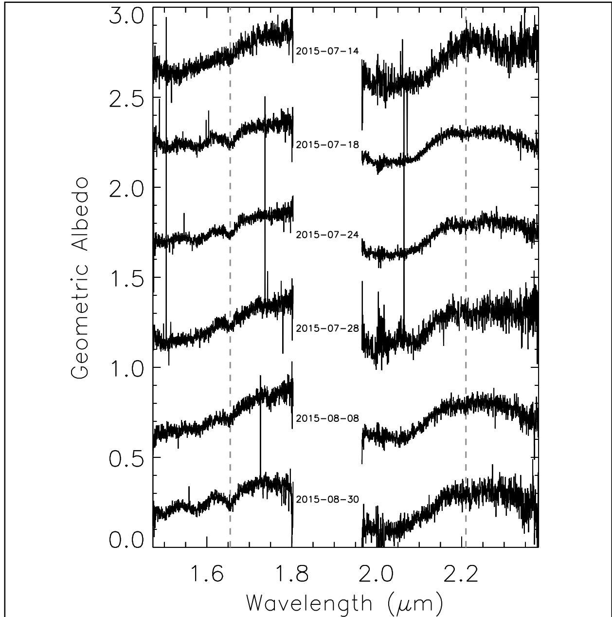
Figure 4: Charon night averaged spectra computed as robust averages ( 3\text{-}\sigma ) of the reduced spectra from each given night (dates are marked between each H and K pair). The spectra are offset in intervals of 0.5 in geometric albedo for clarity. Vertical dashed lines mark the approximate centers of the 1.65\ \mu\text{m} crystalline water ice band and the 2.21\ \mu\text{m} ammonia hydrate band. The highest signal-to-noise spectra were obtained on 2015-07-18 and 2015-07-24, and these two nights dominate the grand average (calculated using a weighted average).
