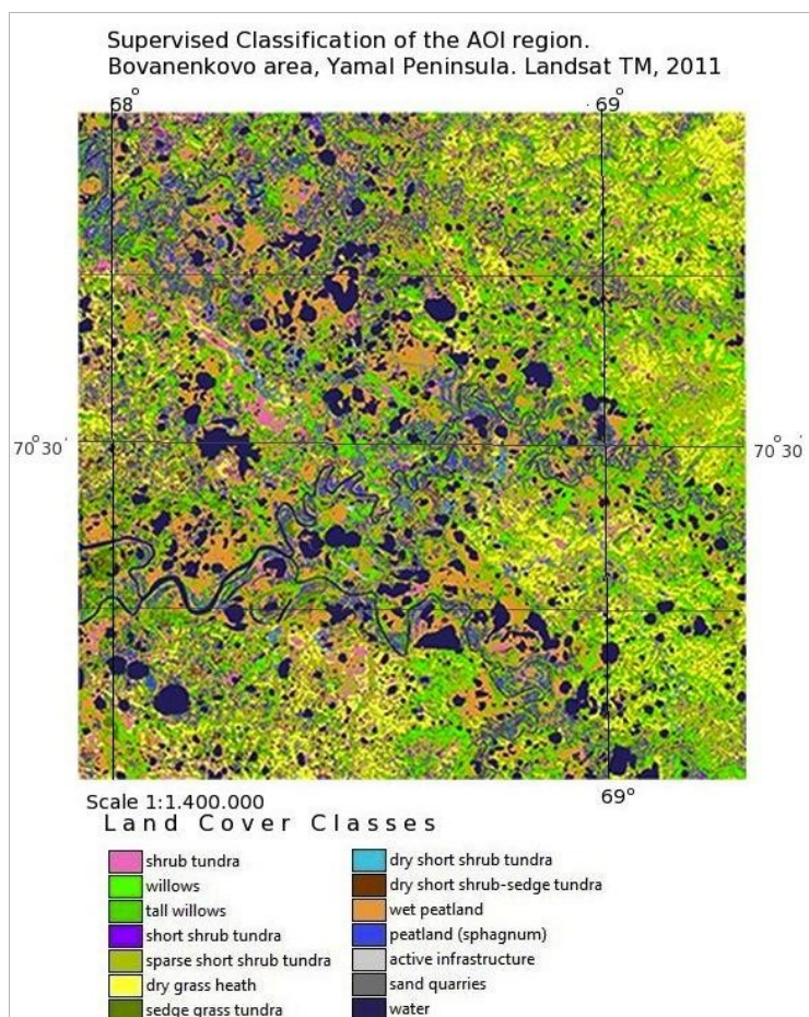
Figure 1 Land cover classes in AOI (Area Of Interest): Bovanenkovo region, Yamal. Results of the supervised classification of the Landsat TM image, 2011 performed in ILWIS GIS
