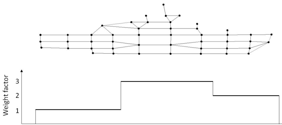
Figure 6: Weight factors for different longitudinal positions
