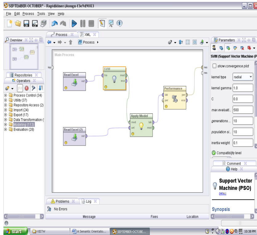
Figure 2. Classification model using SVM-PSO
