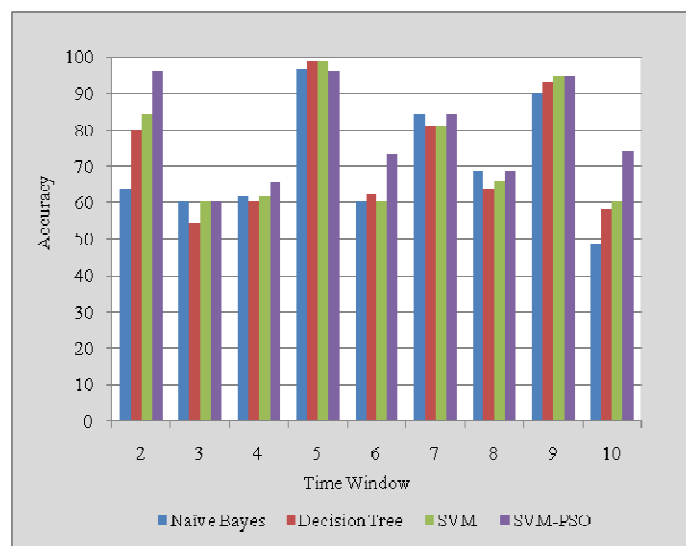
Figure 3. Accuracy comparison while using SVM-PSO and other algorithms
