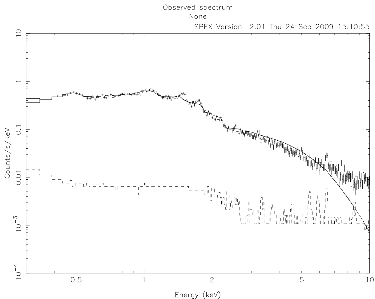
Figure 7.3: A fit without modeling the particle background is not successful. Especially, the high-energy region in the spectrum is not fitted well due to soft protons.
