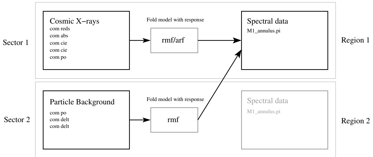
Figure 7.1: Schematic representation of the sectors and regions in this example. We load two spectra with trafo and we define two sectors (left). The exact model components are later defined in SPEX . The models for sectors 1 and 2 are folded through the response matrix separately. The result of the folding is added and applied to the first spectrum (region 1 on the right) only.
