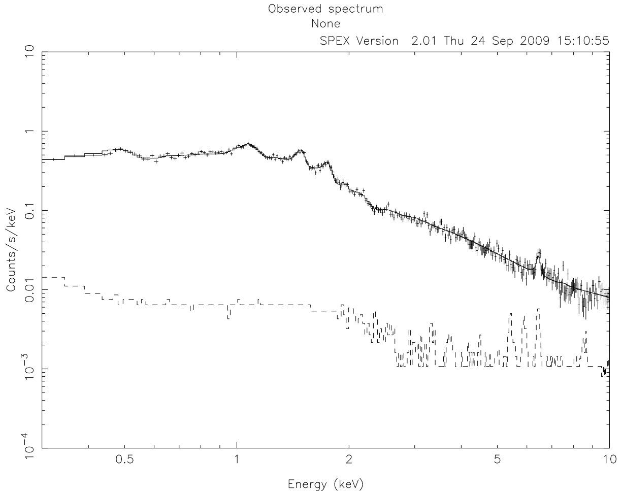
Figure 7.5: Best fit model to our example spectrum. The particle background model has been able to fit the discrepancies at high energies.
