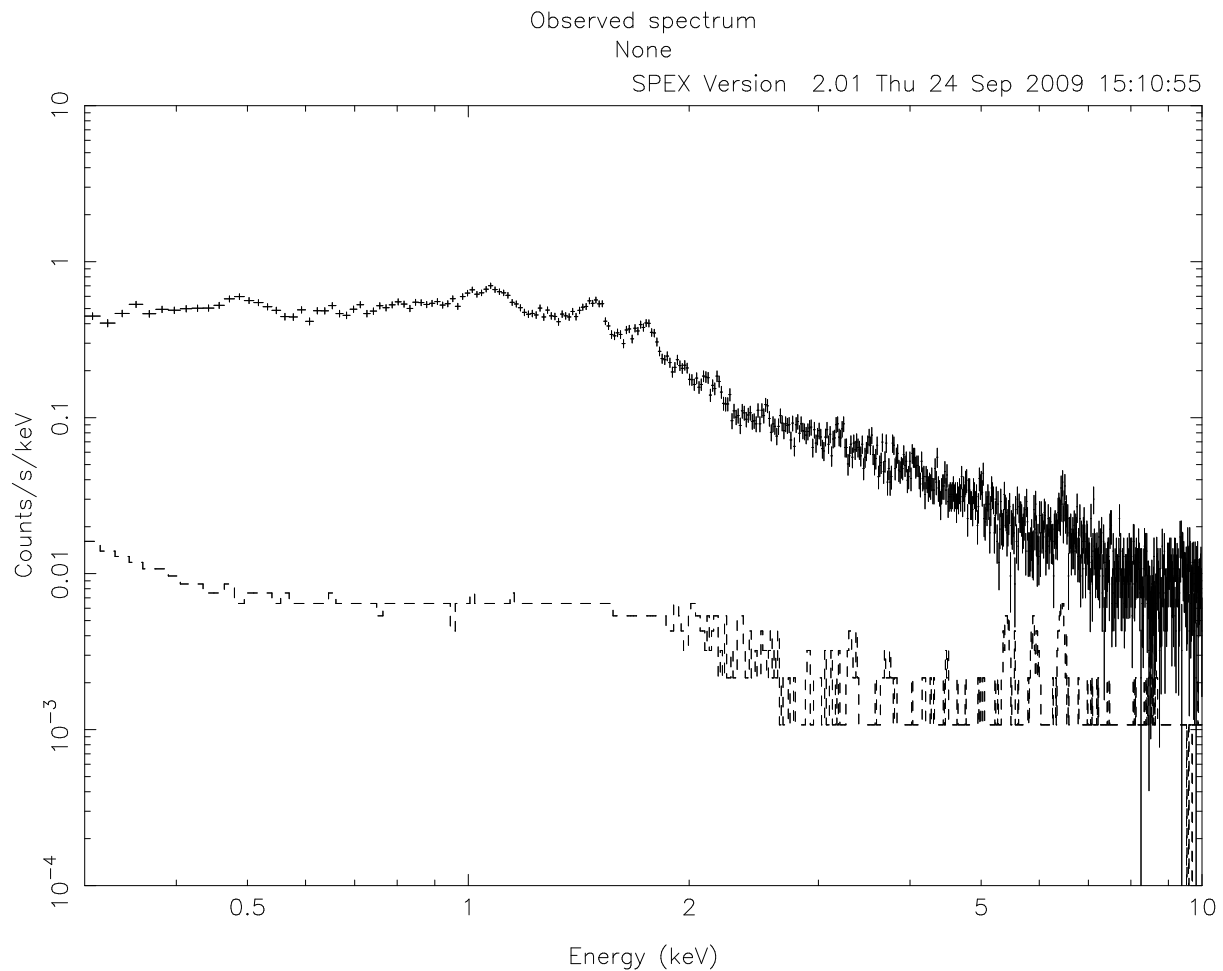
Figure 7.2: XMM-Newton MOS1 spectrum extracted from a 6–9 arcmin annulus around a cluster of galaxies.
