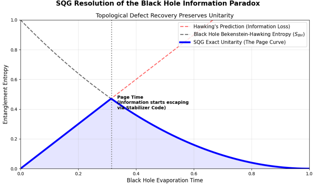
Figure 3: Numerical simulation of the Black Hole Information Paradox resolution in SQG. The solid blue line tracks the exact Page Curve, where the activation of the Stabilizer Code at t_P prevents information loss and restores Unitarity.
