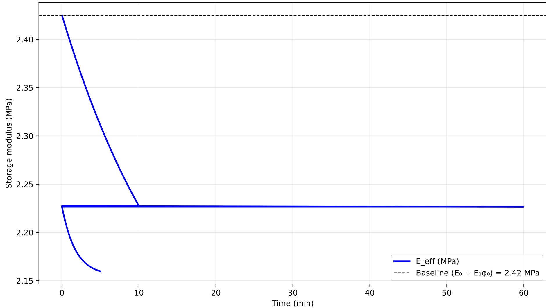
Predicted modulus evolution during training / rest / erasing
