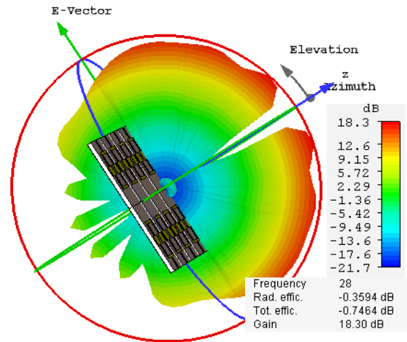
Fig. 8 (a) 3D Array gain with end-fire on azimuth plane
