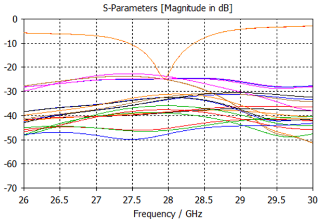
Fig. 7 Port isolations S11, S21, S31, etc.
