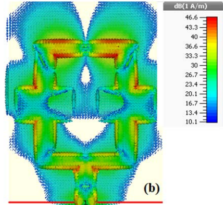
Fig. 3 Simulated (a) radiation pattern characteristics of the antenna at 38 GHz and (b) current distribution
