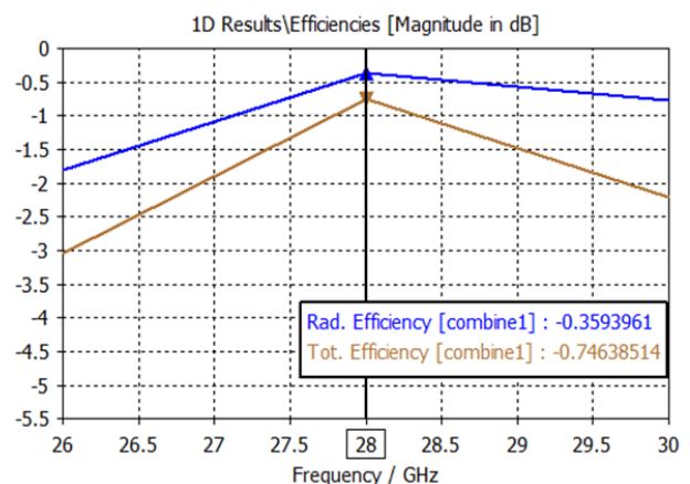
Fig. 9 Radiation and Total Efficiency of Array Antenna
