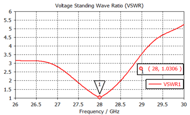
Fig. 4 Voltage standing wave ratio of single element antenna
