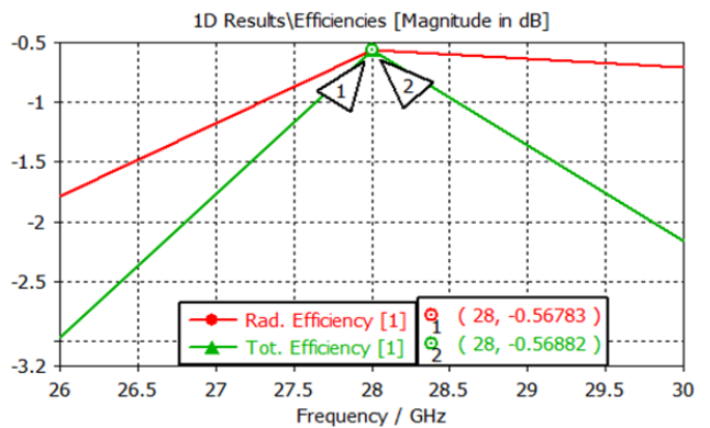
Fig. 5 Radiation and total efficiency of single antenna
