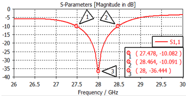
Fig. 2 Return loss of single element antenna
