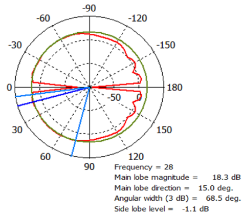
Fig. 8 (b) Array gain polar radiation on azimuth plane
