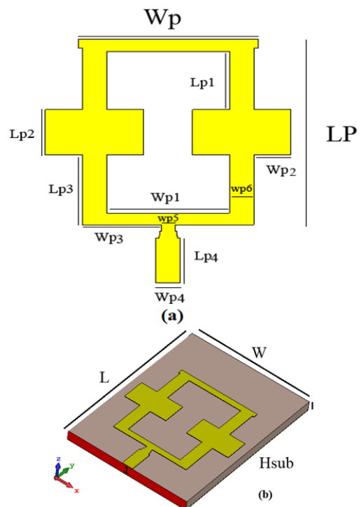
Fig. 1 Dimension of single element (a) Patch (b) sub array antenna
