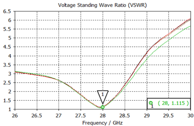
Fig. 10 Voltage Standing Wave Ratio array 8x2 antenna
