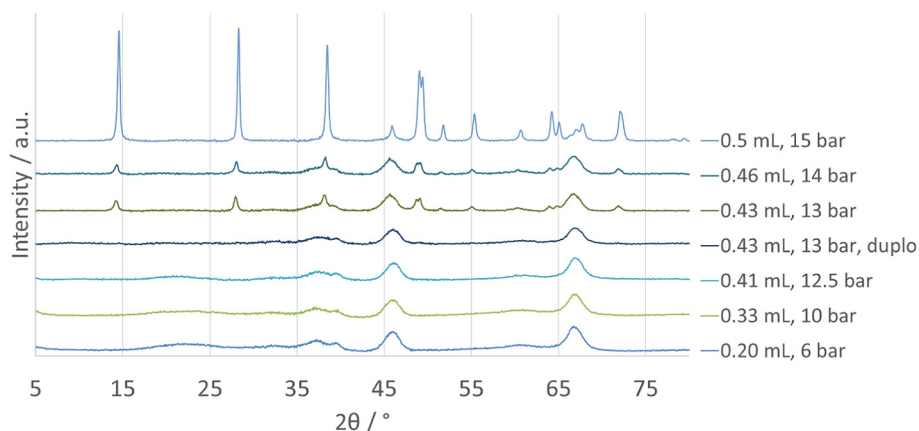
Fig. 2. PXRD measurements of \gamma -Al 2 O 3 after 18.5 h exposure to 250 °C, 6–15 bar H 2 O.
