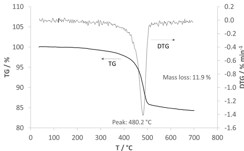
Fig. 3. The TGA curve of the \gamma -Al 2 O 3 sample exposed to steam at 14 bar for 6 h.
