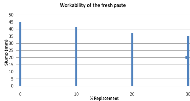
Figure 3: Graph of slump (mm) against % replacement
